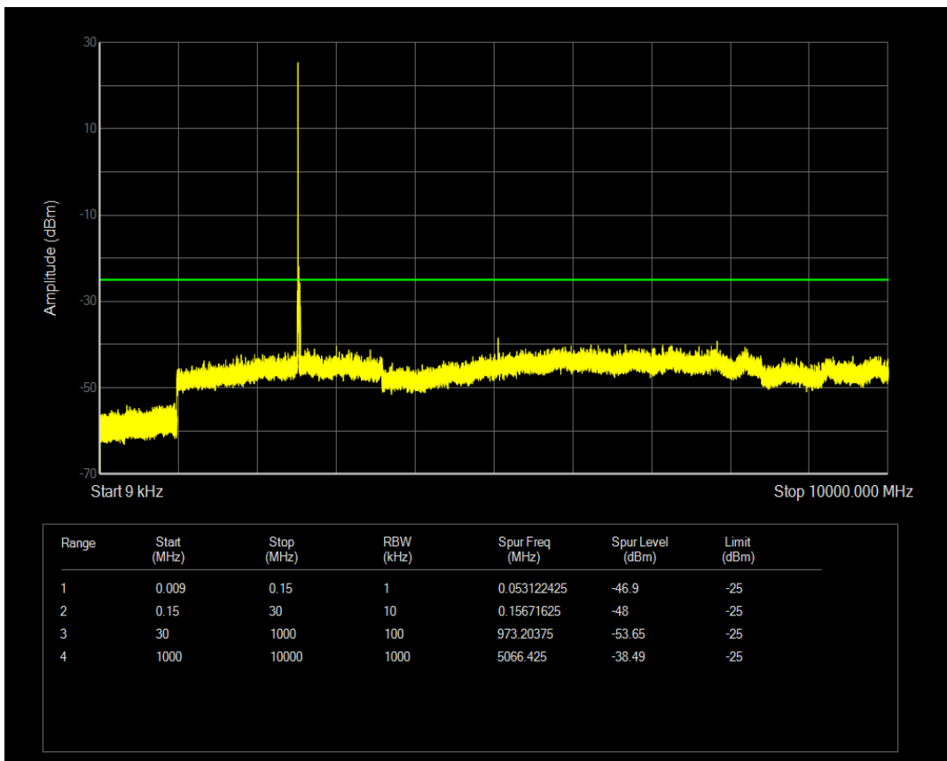
Band7 QAM16 BW=5MHz Channel=21100 RB Size=1 Position=#Max
