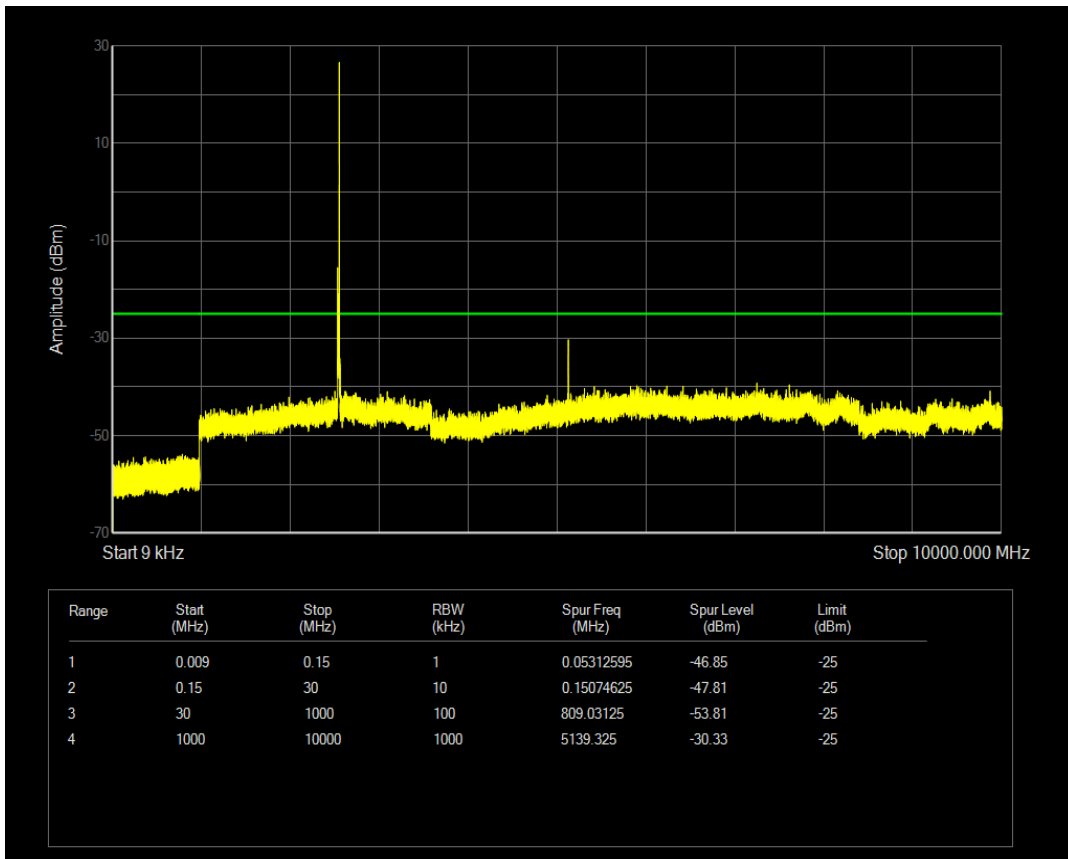
Band7 QPSK BW=10MHz Channel=21400 RB Size=25 Position=#0
