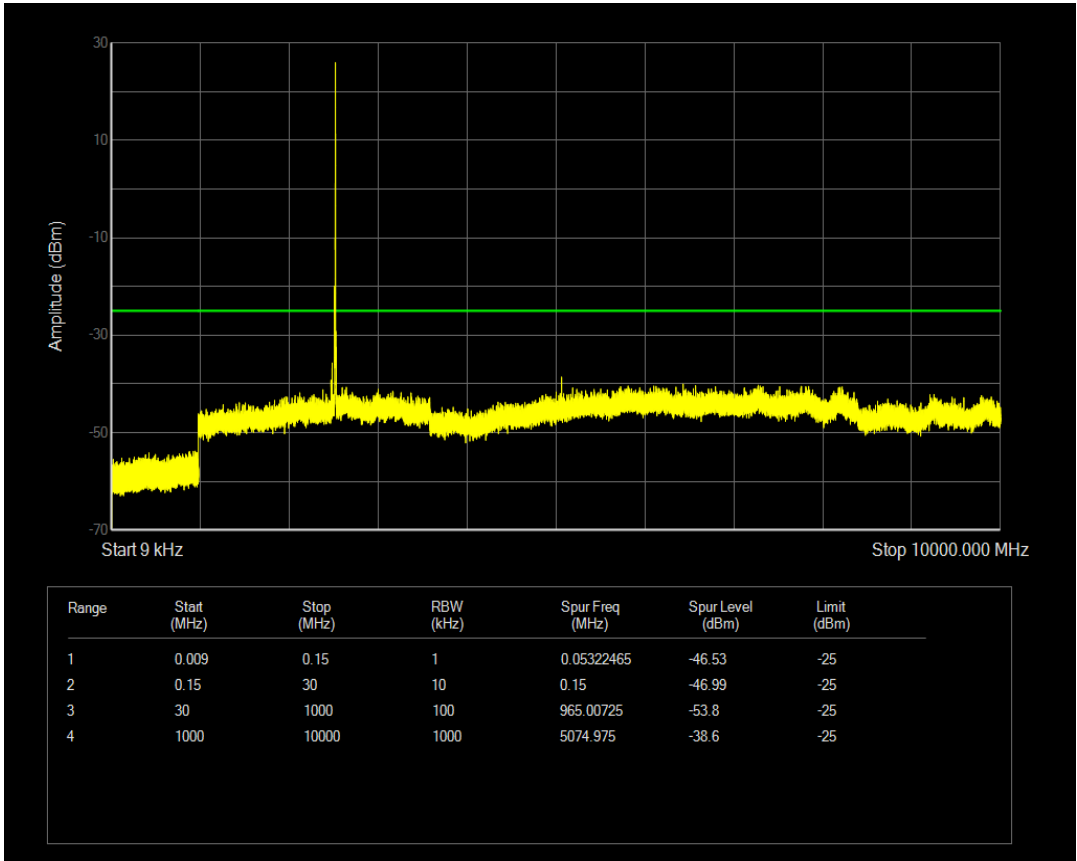
Band7 QAM16 BW=5MHz Channel=21100 RB Size=12 Position=#0
