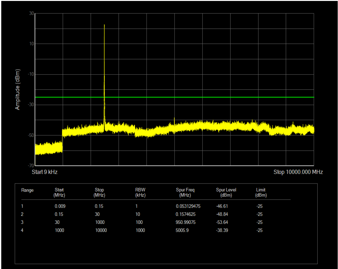
Band7 QPSK BW=10MHz Channel=20800 RB Size=25 Position=#Max
