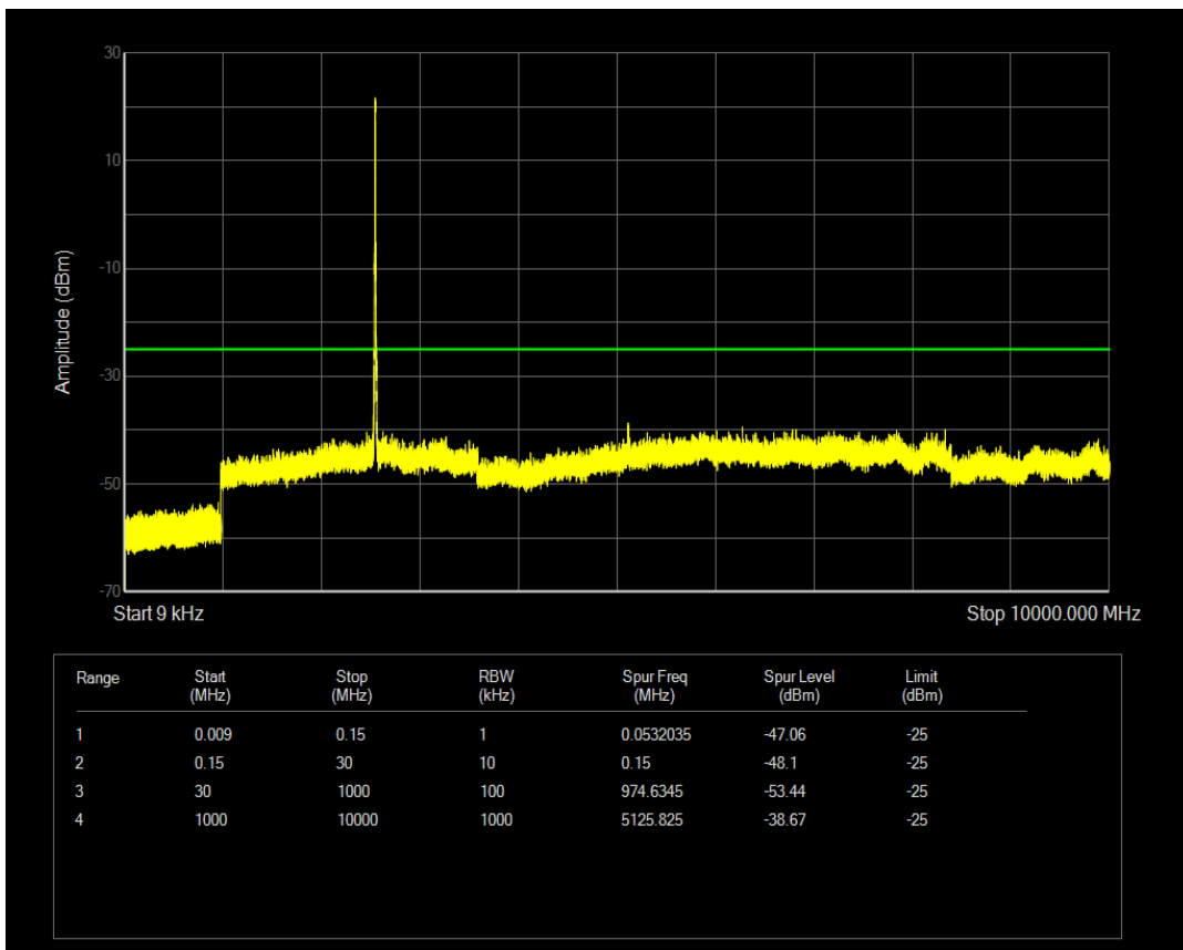
Band7 QAM16 BW=10MHz Channel=21400 RB Size=25 Position=#Max
