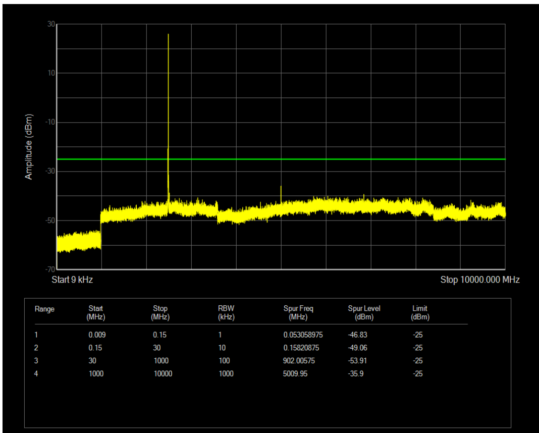
Band7 QAM16 BW=5MHz Channel=20775 RB Size=12 Position=#0
