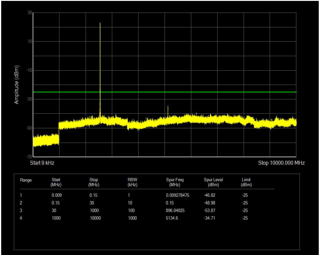
Band7 QAM16 BW=5MHz Channel=21425 RB Size=12 Position=#Max
