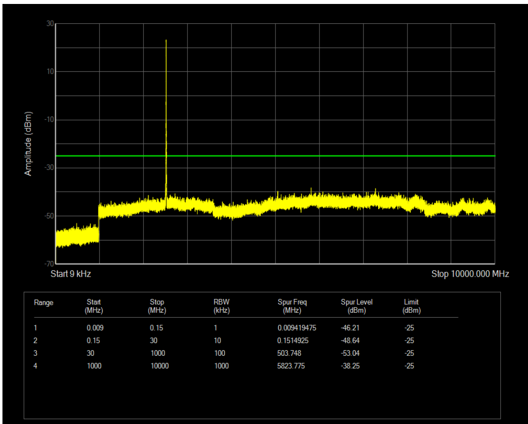
Band7 QPSK BW=5MHz Channel=21100 RB Size=12 Position=#Max
