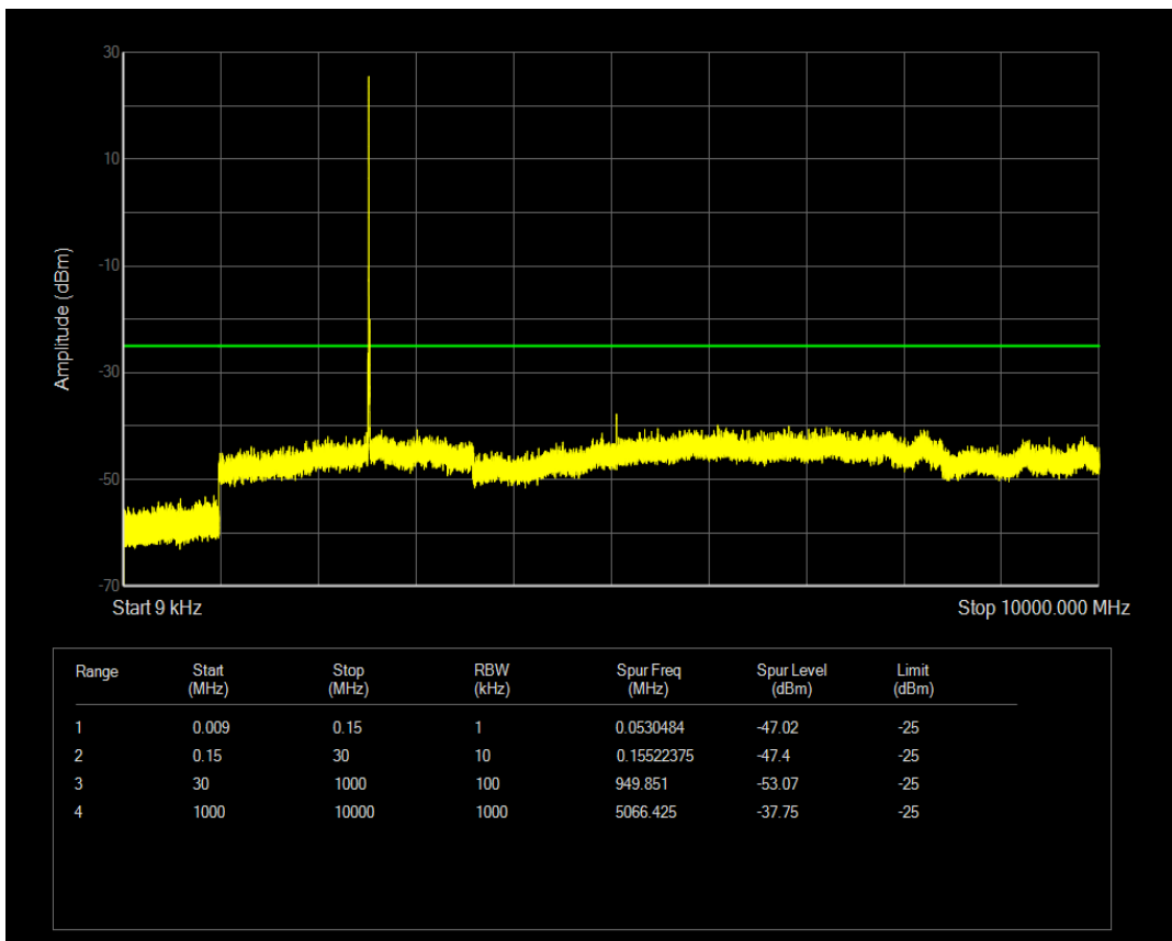
Band7 QPSK BW=5MHz Channel=21100 RB Size=1 Position=#Max
