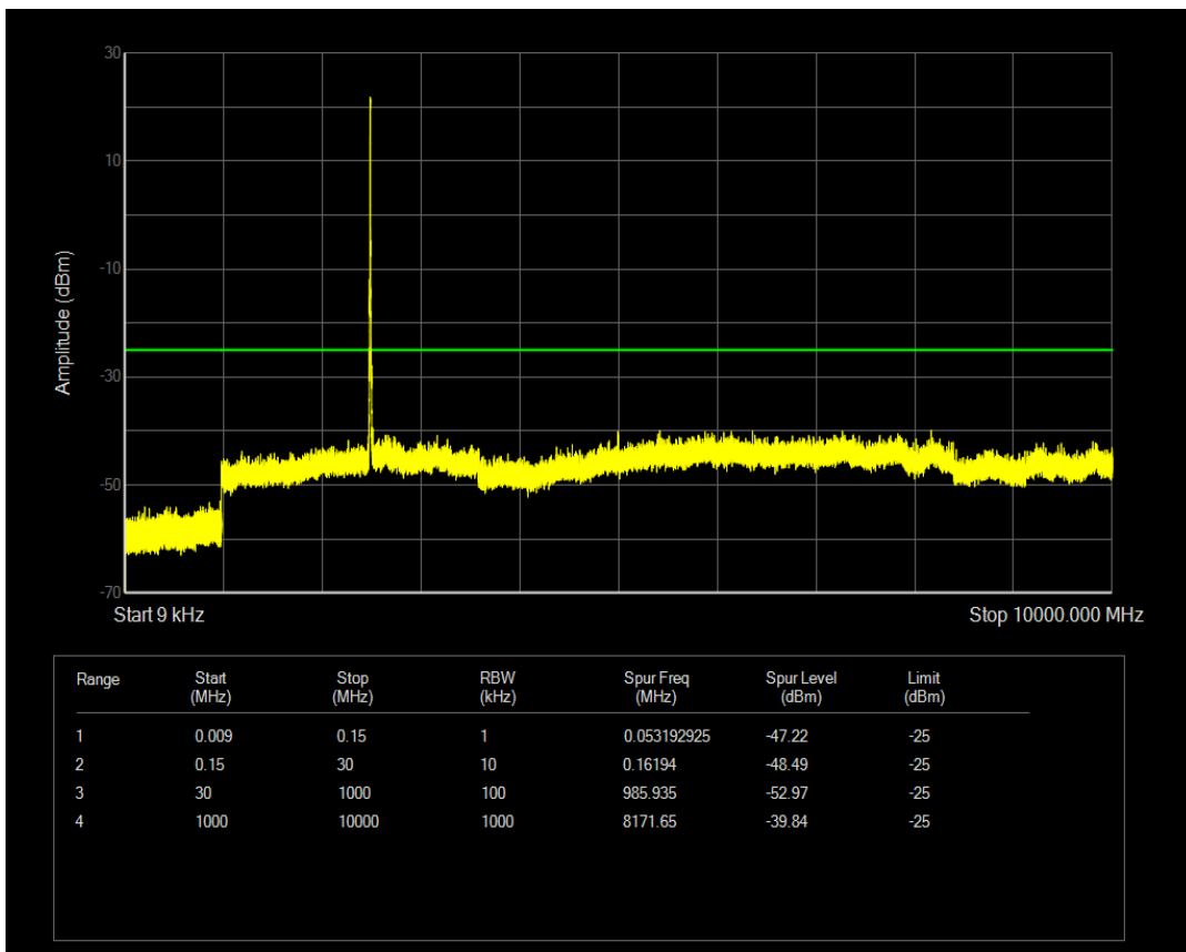
Band7 QAM16 BW=10MHz Channel=20800 RB Size=25 Position=#Max
