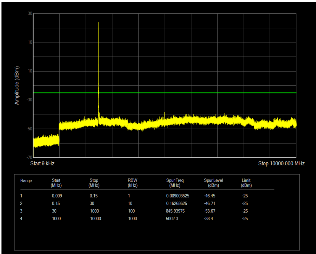
Band7 QAM16 BW=5MHz Channel=20775 RB Size=12 Position=#Max
