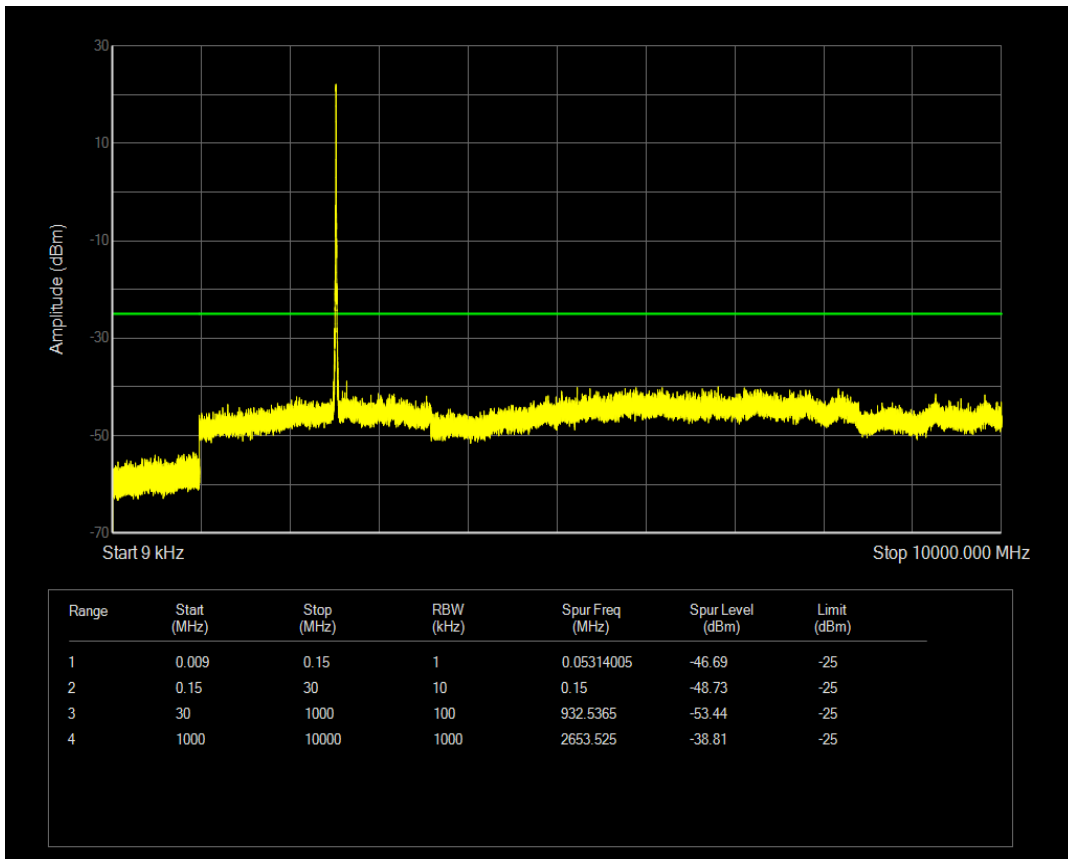
Band7 QPSK BW=10MHz Channel=21100 RB Size=25 Position=#Max
