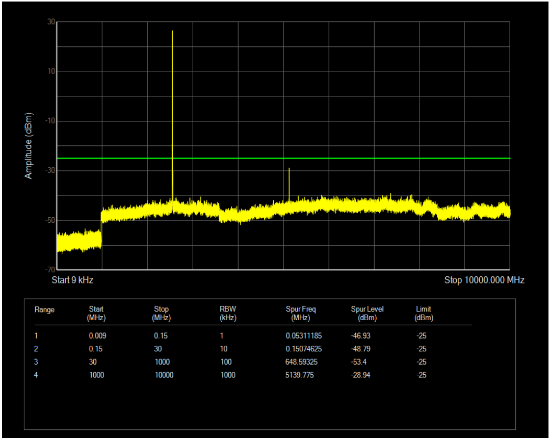
Band7 QAM16 BW=5MHz Channel=21425 RB Size=12 Position=#0
