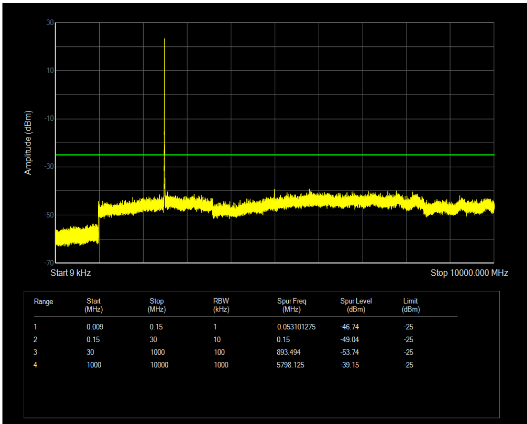
Band7 QPSK BW=5MHz Channel=20775 RB Size=12 Position=#Max
