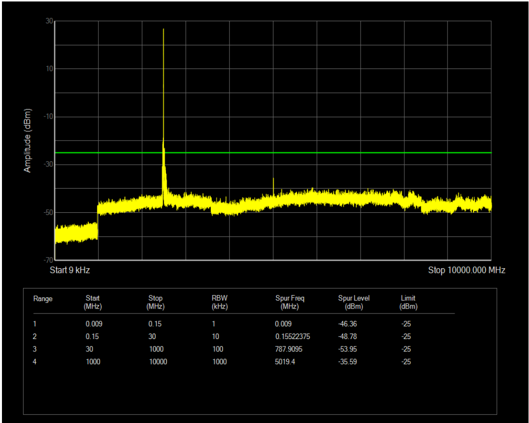
Band7 QPSK BW=10MHz Channel=20800 RB Size=25 Position=#0
