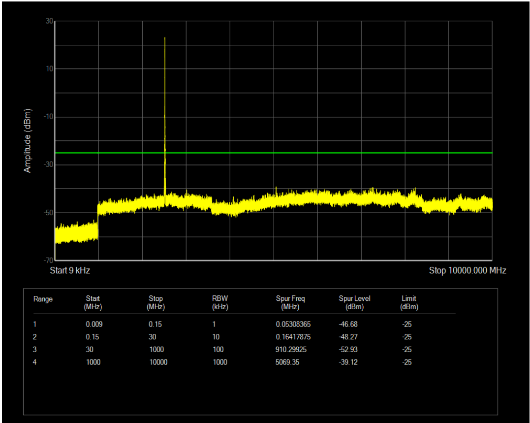
Band7 QAM16 BW=5MHz Channel=21100 RB Size=12 Position=#Max
