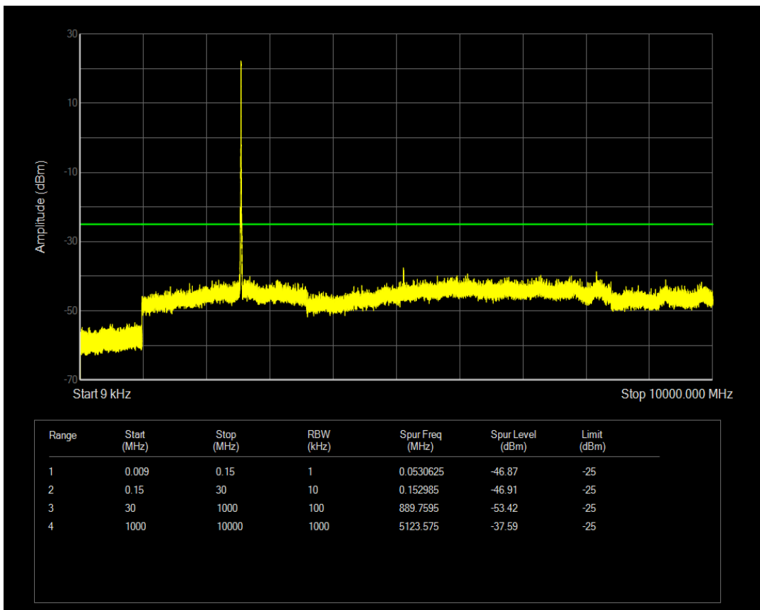
Band7 QPSK BW=10MHz Channel=21400 RB Size=25 Position=#Max
