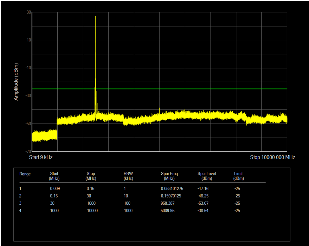
Band7 QPSK BW=5MHz Channel=20775 RB Size=12 Position=#0
