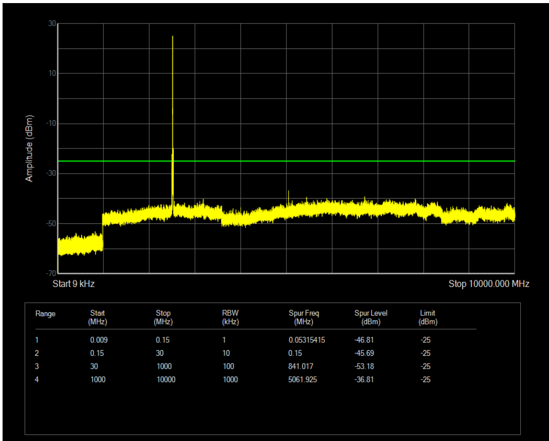
Band7 QPSK BW=10MHz Channel=21100 RB Size=1 Position=#Max
