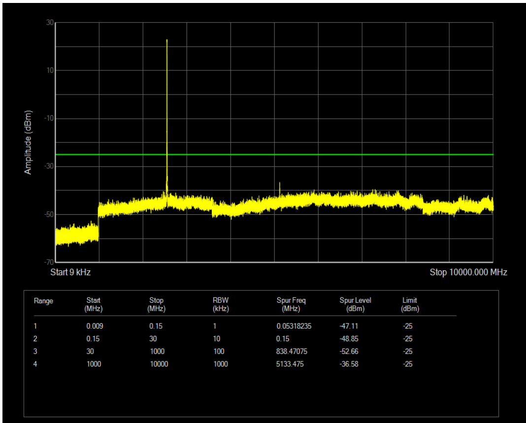
Band7 QPSK BW=5MHz Channel=21425 RB Size=12 Position=#Max
