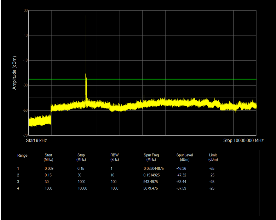
Band7 QAM16 BW=10MHz Channel=21100 RB Size=25 Position=#0
