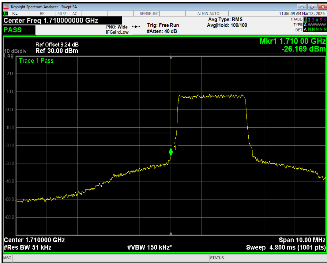
Band4 QPSK BW=5MHz Channel=19975 RB Size=12 Position=#Max
