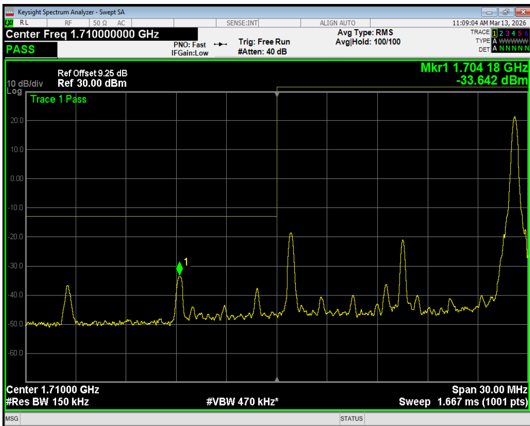
Band4 QPSK BW=15MHz Channel=20025 RB Size=36 Position=#0
