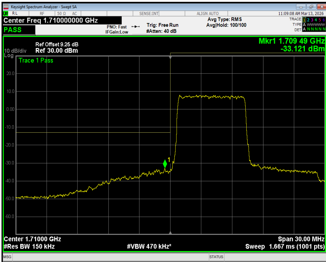
Band4 QPSK BW=15MHz Channel=20025 RB Size=36 Position=#Max
