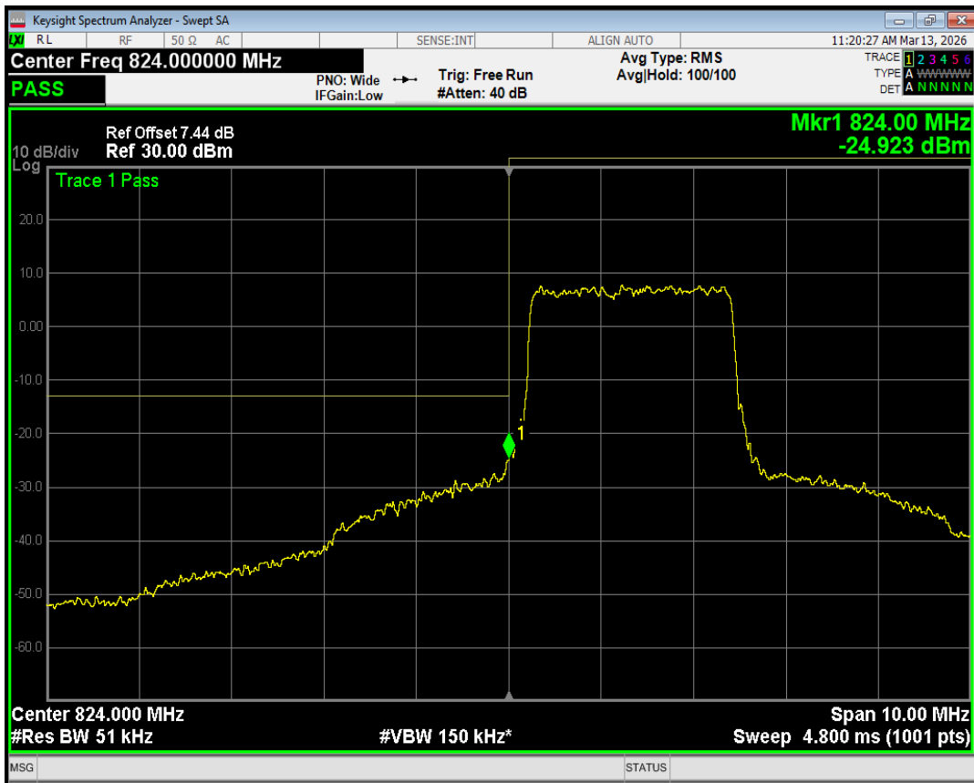
Band5 QPSK BW=5MHz Channel=20425 RB Size=12 Position=#Max
