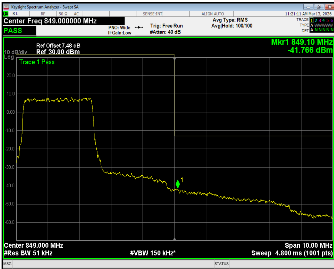
Band5 QPSK BW=5MHz Channel=20625 RB Size=12 Position=#Max
