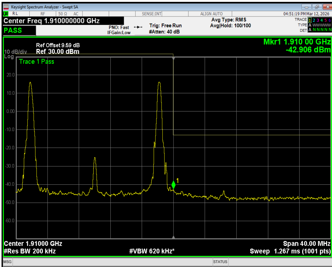
Band2 QAM16 BW=20MHz Channel=19100 RB Size=50 Position=#Max
