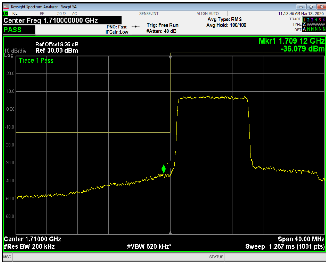
Band4 QPSK BW=20MHz Channel=20050 RB Size=50 Position=#Max
