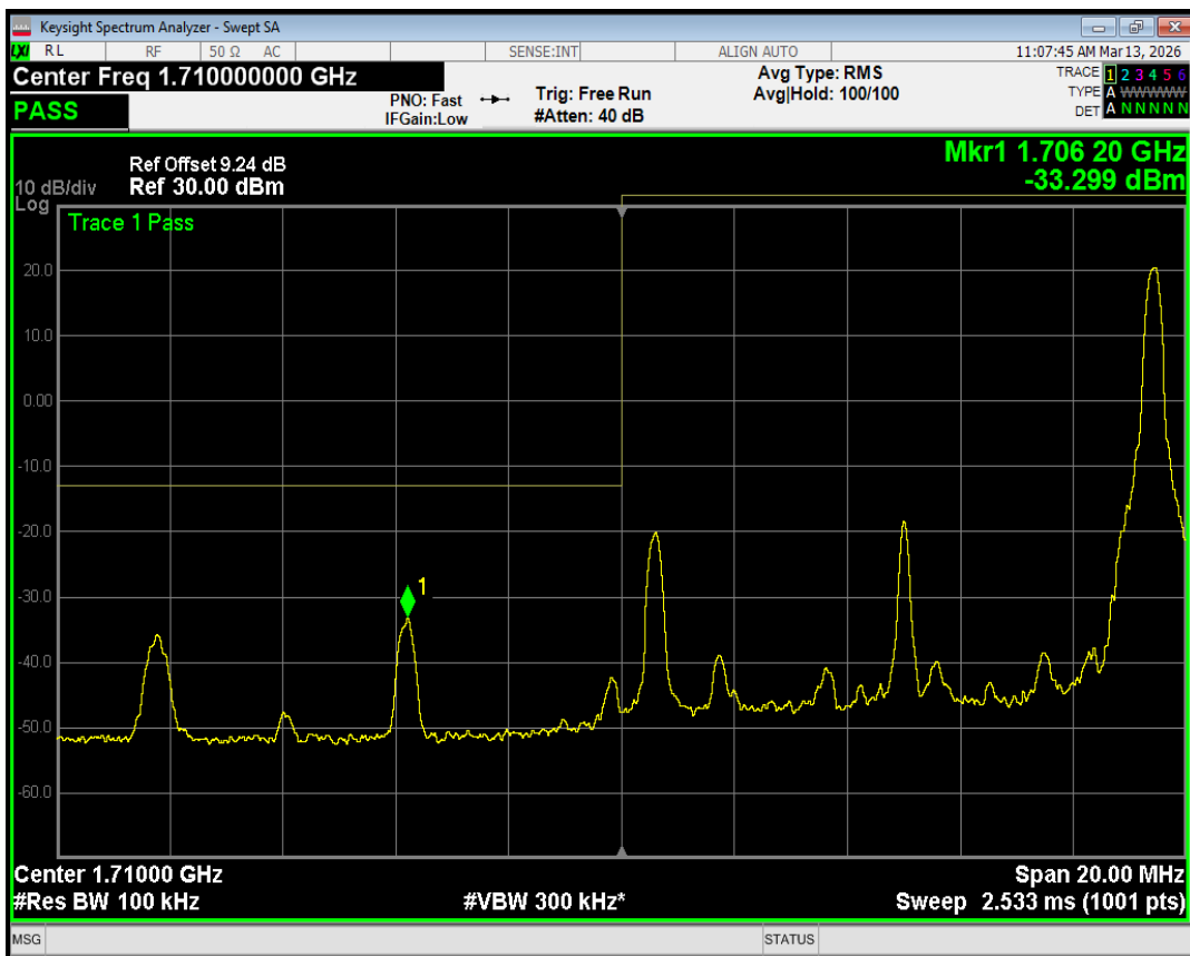
Band4 QPSK BW=10MHz Channel=20000 RB Size=25 Position=#0
