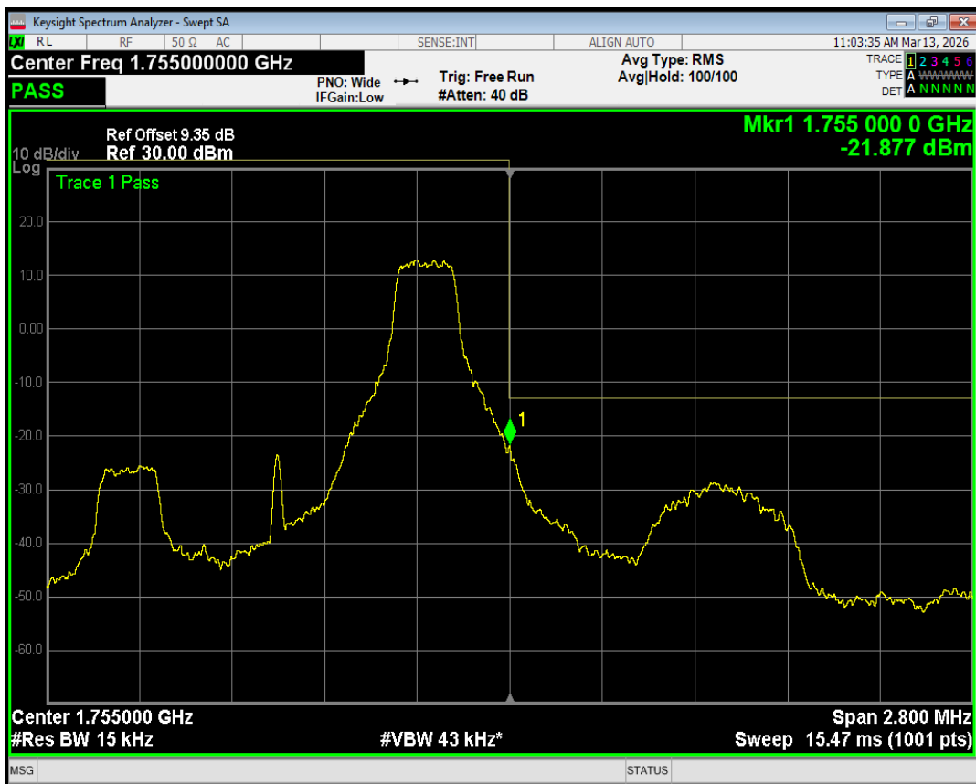
Band4 QPSK BW=1.4MHz Channel=20393 RB Size=3 Position=#0
