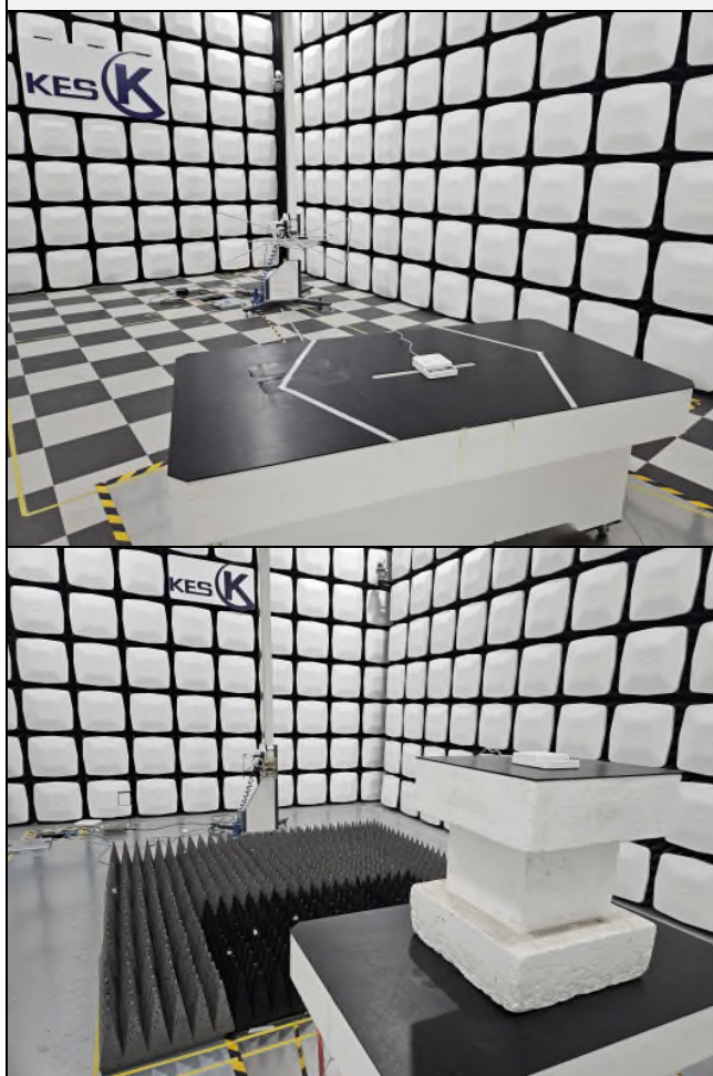
Radiated test
