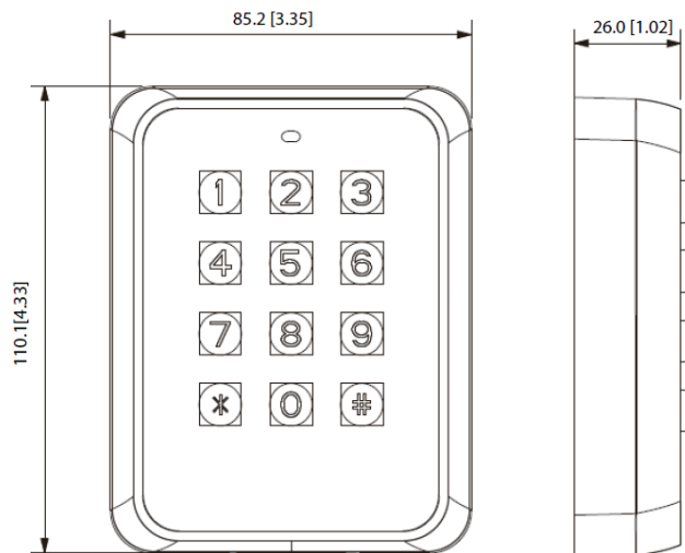
Figure 1-1 Dimensions (unit: mm[inch])
