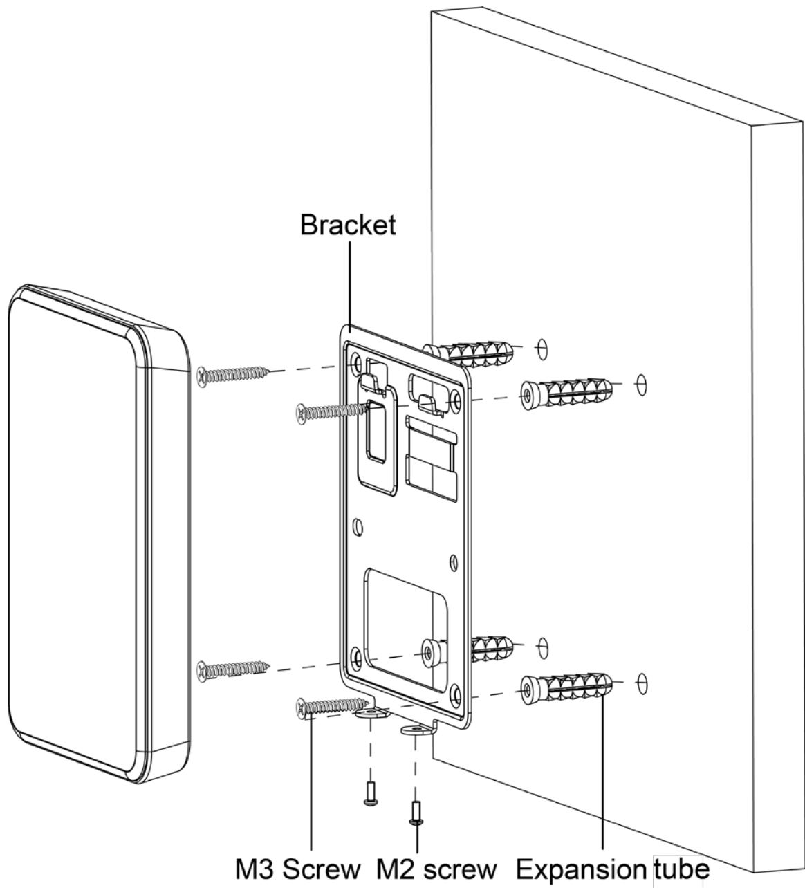
Figure 3-2 Wall mount
