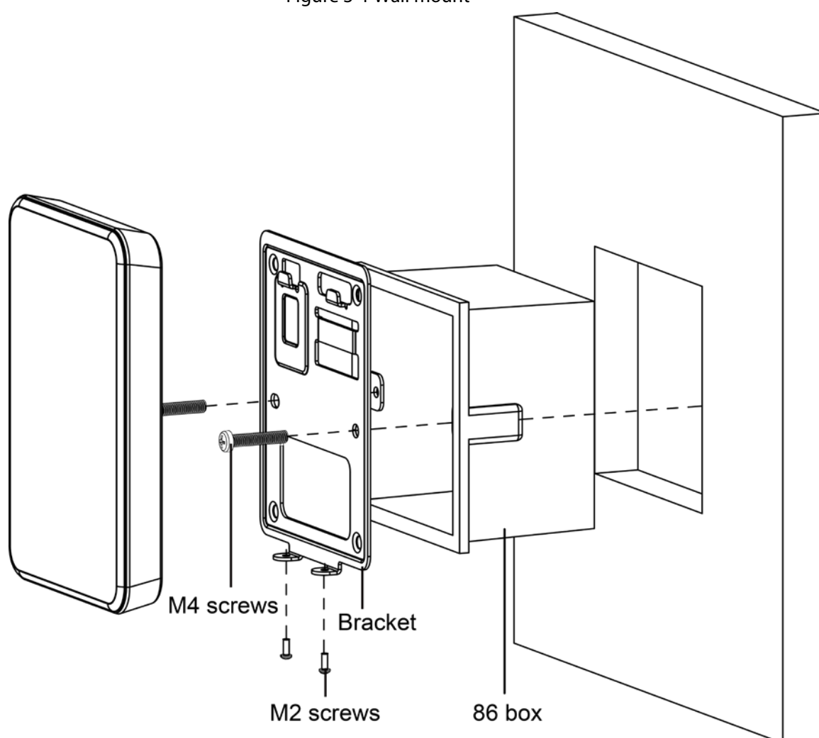
Figure 3-1 Wall mount
