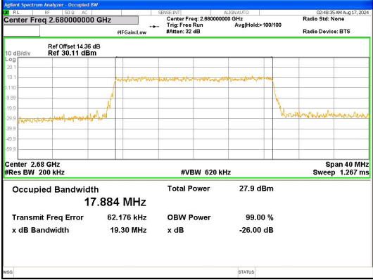
Band 41 20MHz/2680.0/High QPSK 100@0
