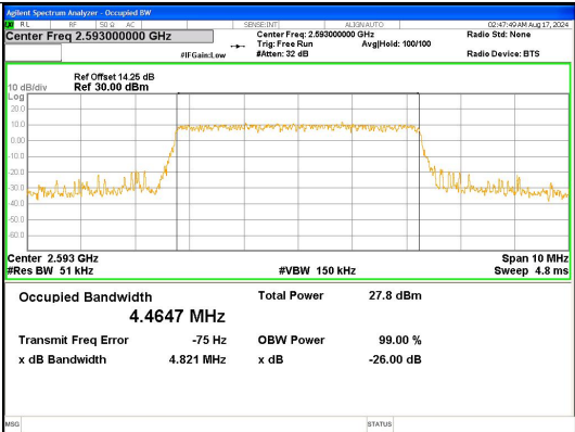
Band 41 5MHz/2593.0/Mid 16QAM 25@0
