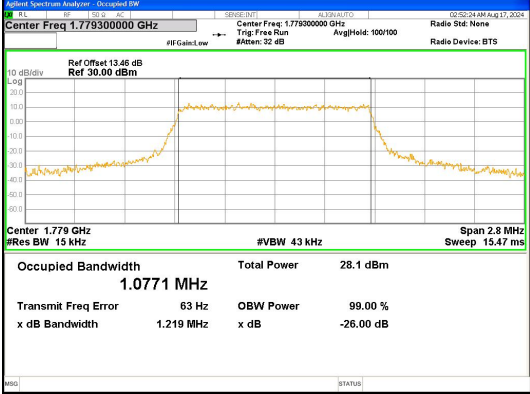
Band 66 1.4MHz/1779.3/High 16QAM 6@0
