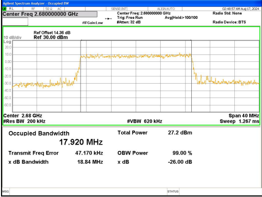
Band 41 20MHz/2680.0/High 16QAM 100@0
