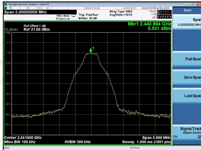
DH5-Ant1-2441-0~Reference-PASS
