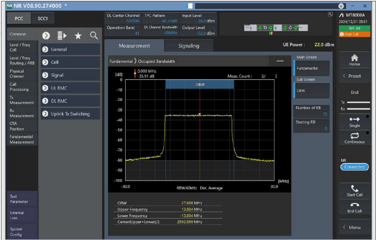
n41_30MHz_30kHz_518598_DFT-s-OFDM QPSK^Outer_Full
