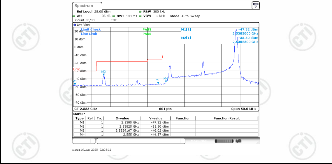
Band41-20MHz-QPSK-40340-1RB#99
