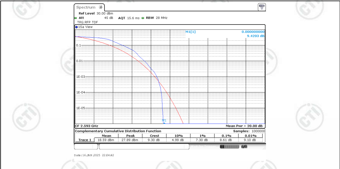
Band41-15MHz-QPSK-40620-1RB#0
