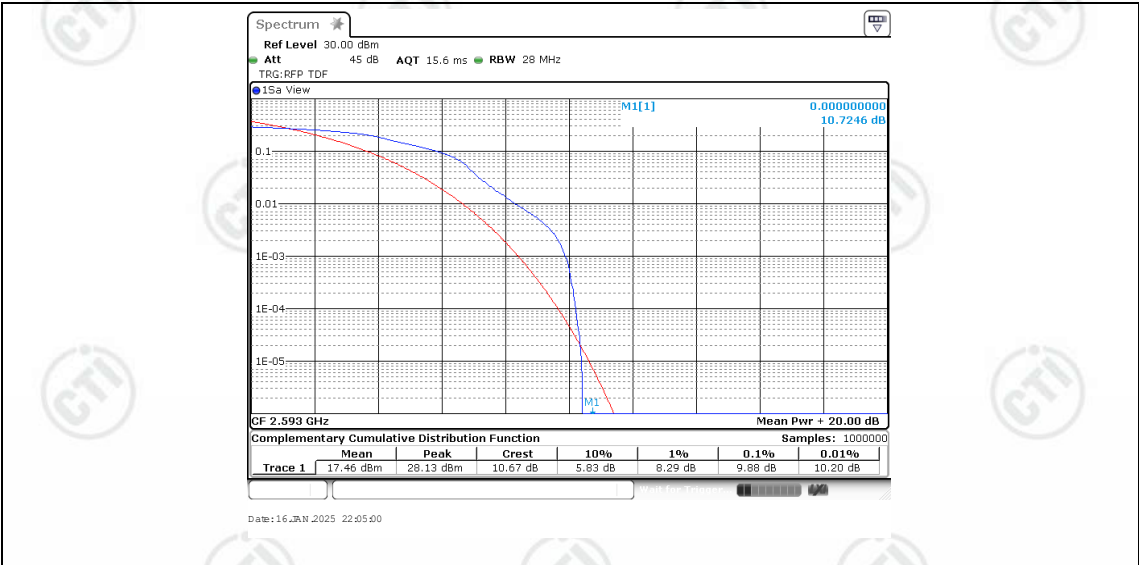
Band41-15MHz-16QAM-40620-1RB#0
