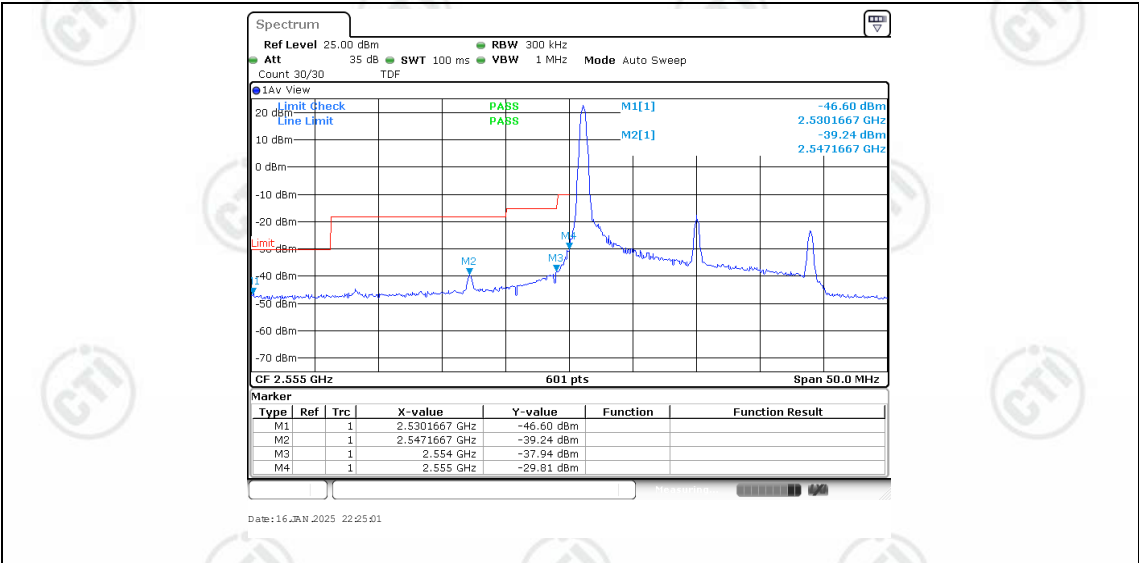
Band41-20MHz-QPSK-40340-1RB#0
