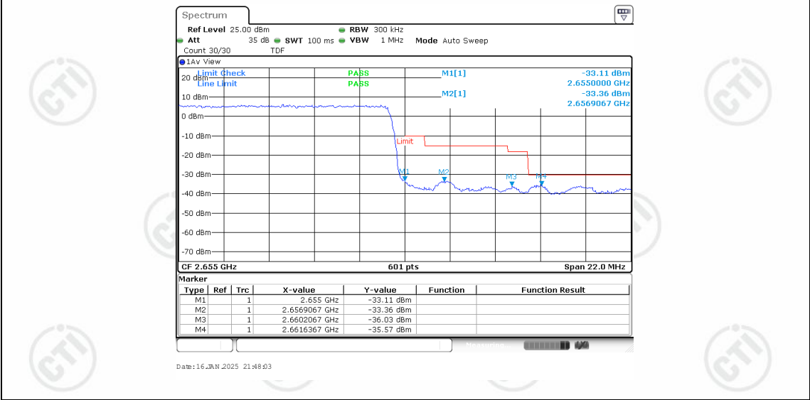
Band41-15MHz-QPSK-41165-75RB#0
