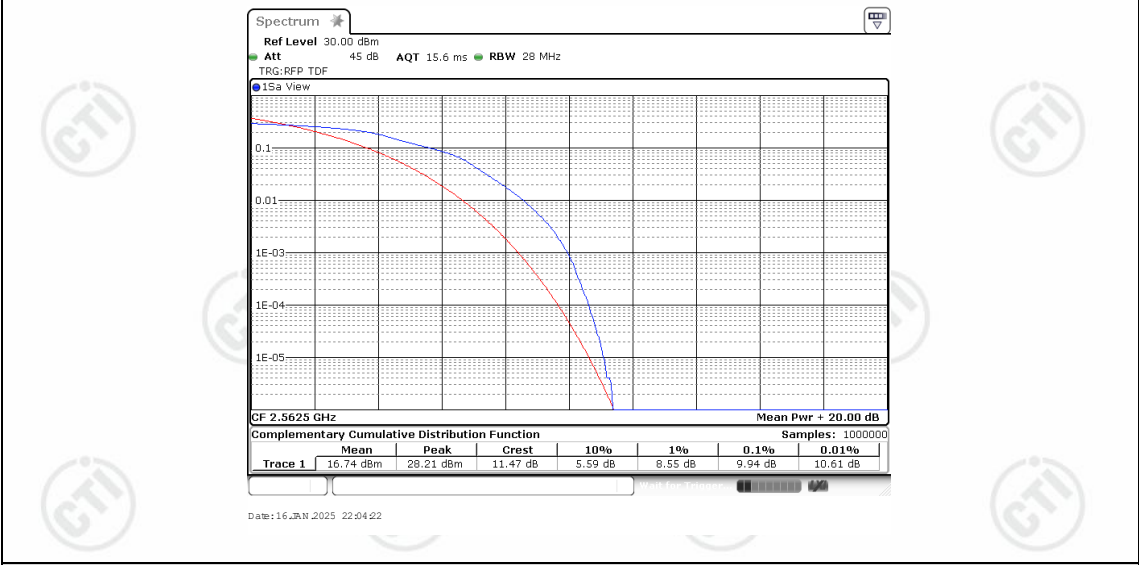
Band41-15MHz-16QAM-40315-75RB#0
