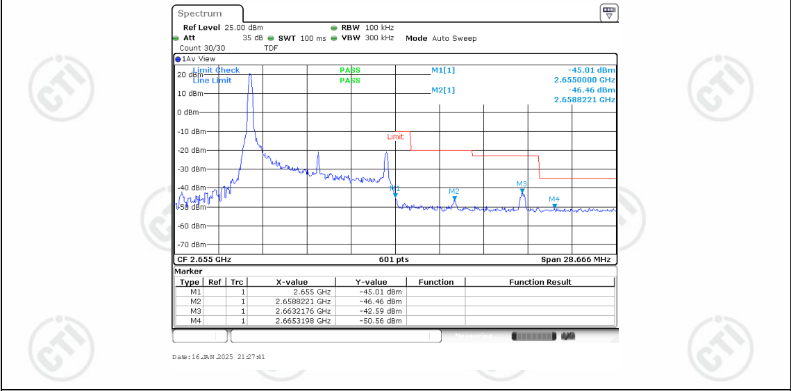
Band41-10MHz-16QAM-41190-1RB#0
