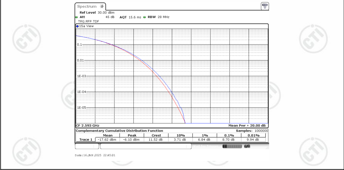
Band41-20MHz-16QAM-40620-100RB#0
