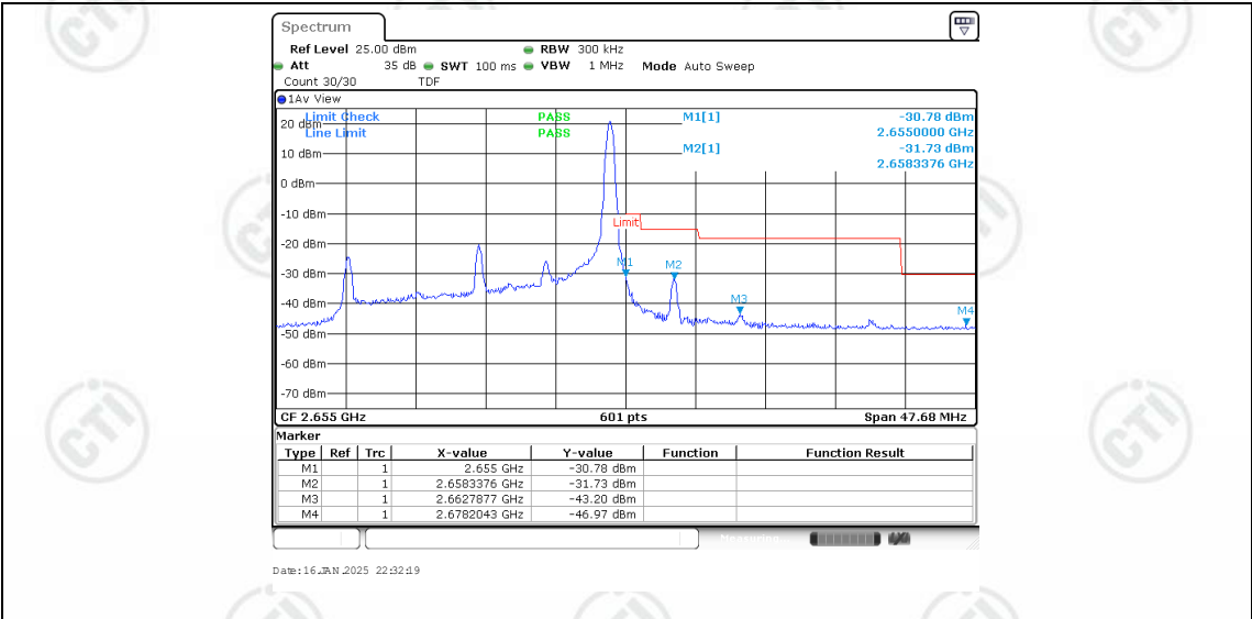
Band41-20MHz-16QAM-41140-1RB#99
