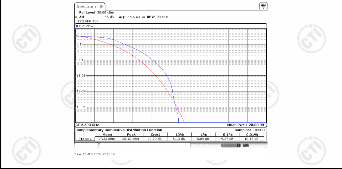
Band41-15MHz-QPSK-40620-75RB#0
