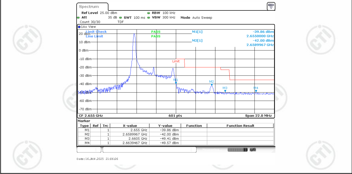
Band41-5MHz-16QAM-41215-1RB#0
