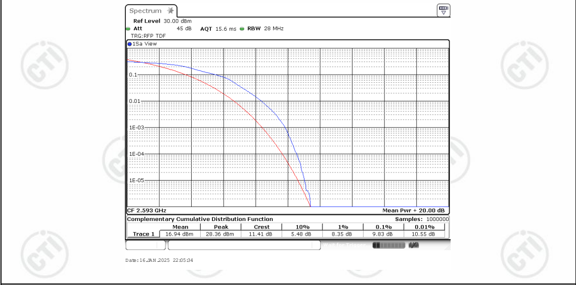
Band41-15MHz-16QAM-40620-75RB#0
