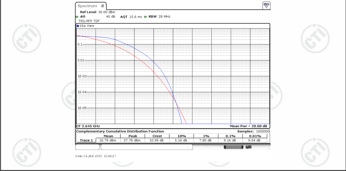
Band41-20MHz-QPSK-41140-100RB#0
