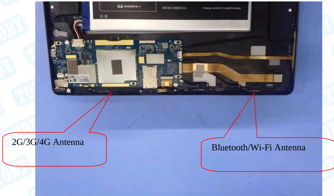
Photo 12 Appearance of PCB
