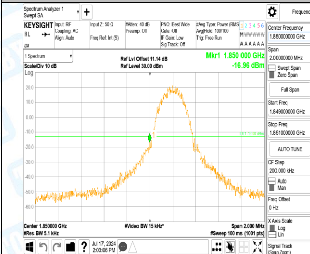
EGPRS1900-512-2-PASS
