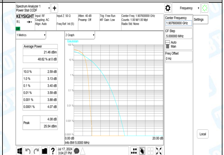
Band2-9538-4-PASS
