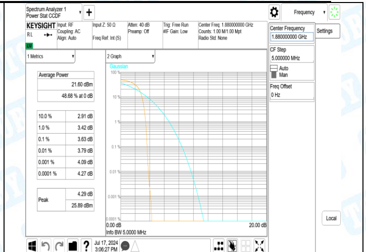
Band2-9538-2-PASS
