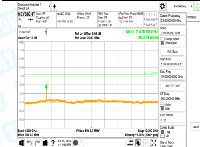
Band5-4132-3-1000~10000MHz-PASS
