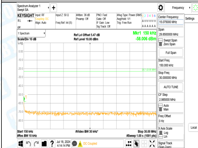
Band5-4182-3-0.15~30MHz-PASS
