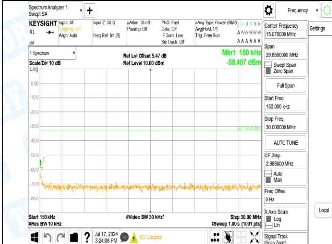
Band2-9538-3-0.15~30MHz-PASS
