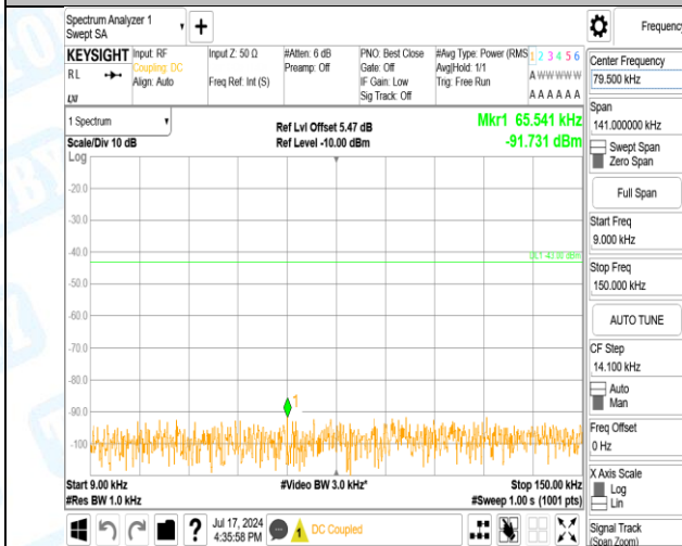
Band2-9400-3-0.009~0.15MHz-PASS
