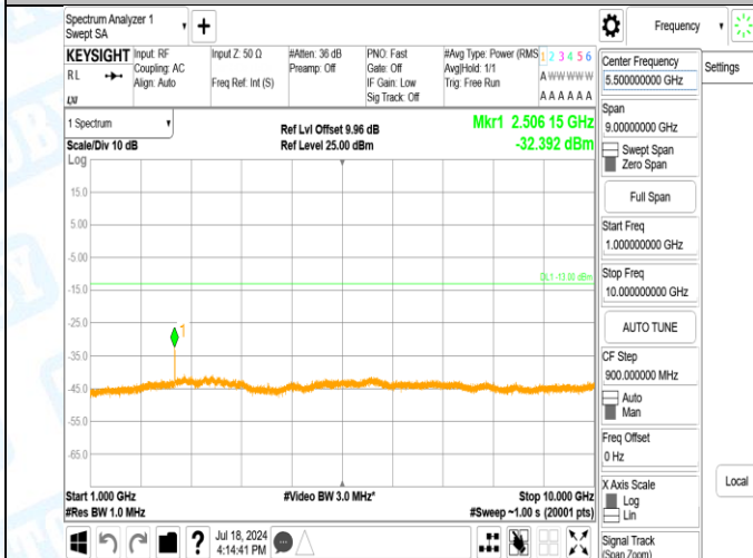
Band5-4182-3-1000~10000MHz-PASS
