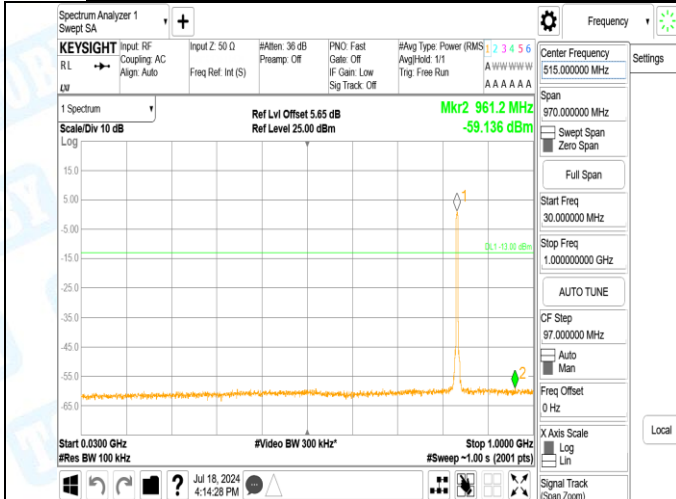
Band5-4182-3-30~1000MHz-PASS
