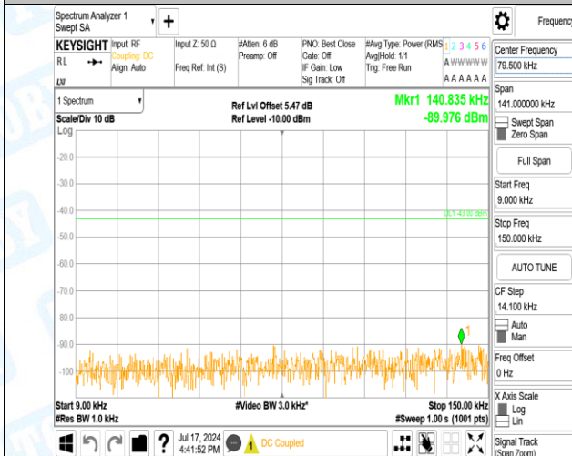
Band2-9400-5-0.009~0.15MHz-PASS
