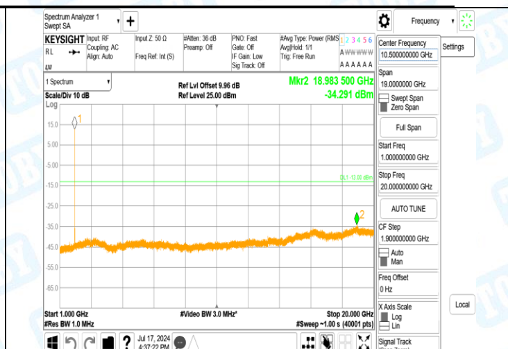
Band2-9538-3-1000~20000MHz-PASS
