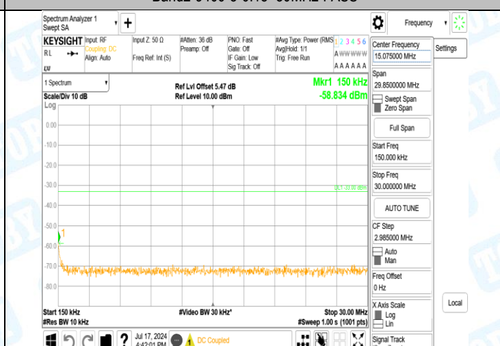
Band2-9400-5-0.15~30MHz-PASS
