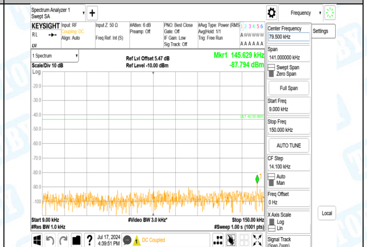
Band2-9538-4-0.009~0.15MHz-PASS
