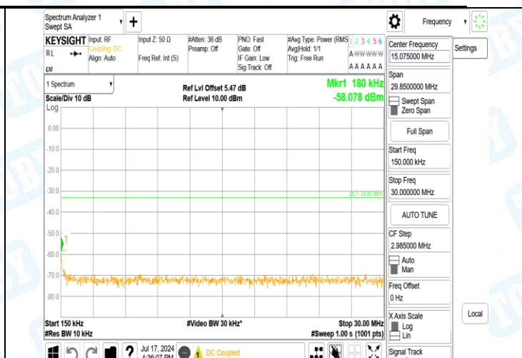
Band2-9400-3-0.15~30MHz-PASS
