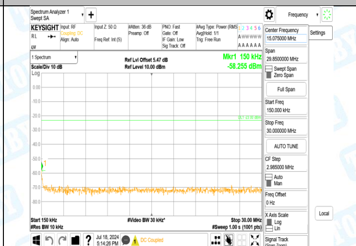
Band5-4132-3-0.15~30MHz-PASS
