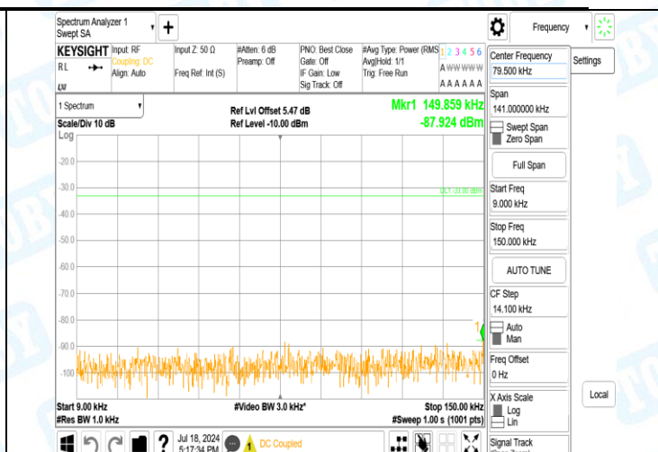
Band5-4132-4-0.009~0.15MHz-PASS
