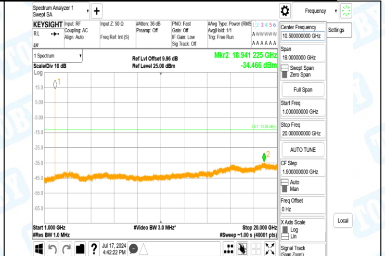
Band2-9400-5-1000~20000MHz-PASS
