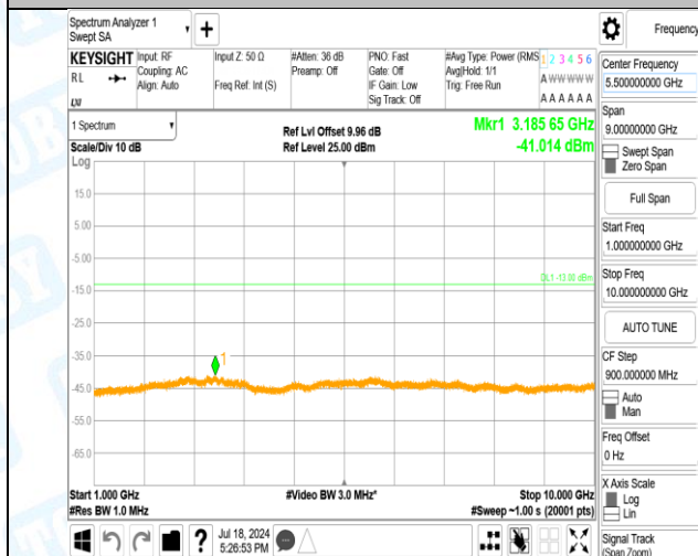
Band5-4233-4-1000~10000MHz-PASS
