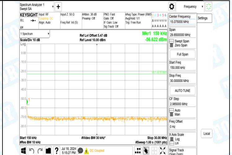
Band5-4182-3-0.15~30MHz-PASS
