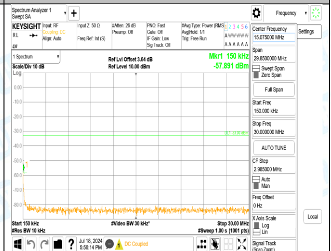
Band2_5MHz_QPSK_19175_1RB#0_1000~3000_1000~3000
