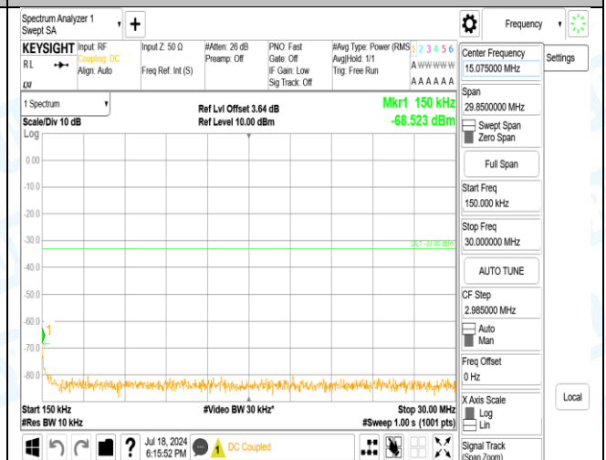
Band2_10MHz_QPSK_19150_1RB#0_1000~3000_1000~3000
