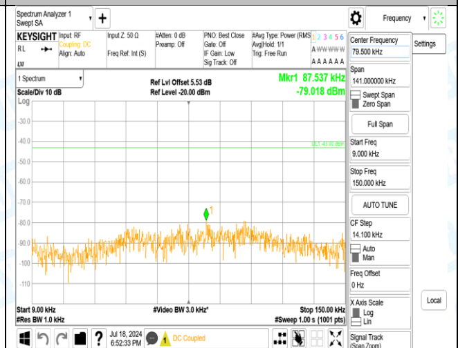
Band2_20MHz_QPSK_18900_1RB#0_30~1000_30~1000
