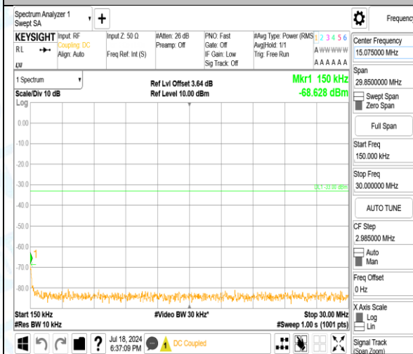
Band2_15MHz_16QAM_19125_1RB#0_1000~3000_1000~3000
