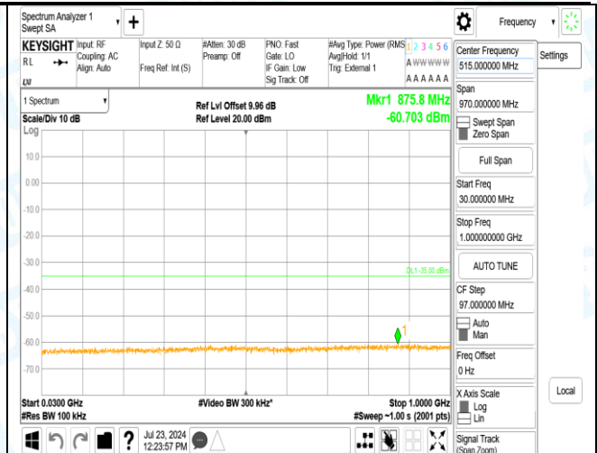
Band38_15MHz_QPSK_38000_1RB#0_20000~27000_20000~27000
