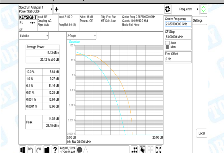
40(2350-2360)-5MHz-16QAM-39175-25RB#0-PASS
