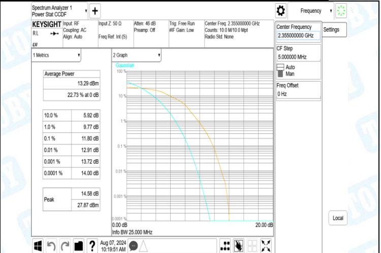
40(2350-2360)-5MHz-16QAM-39225-25RB#0-PASS
