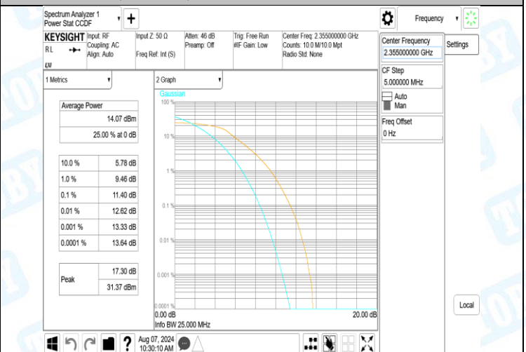
40(2350-2360)-10MHz-16QAM-39200-50RB#0-PASS
