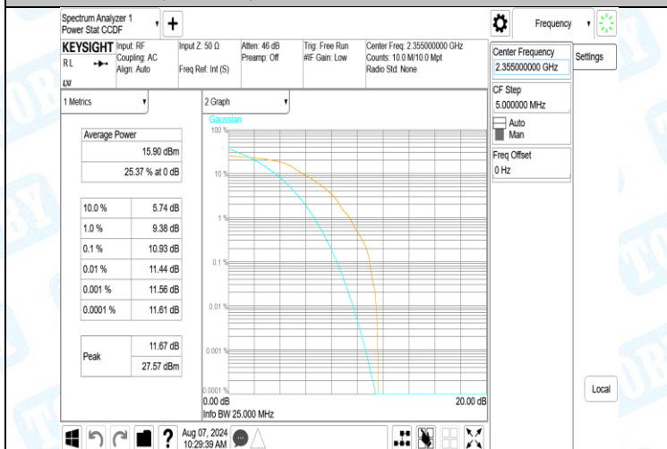
40(2350-2360)-10MHz-16QAM-39200-1RB#0-PASS
