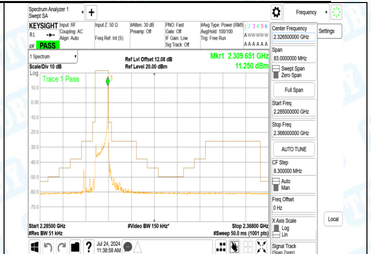
Band40_5MHz_16QAM_38775_1RB#0
