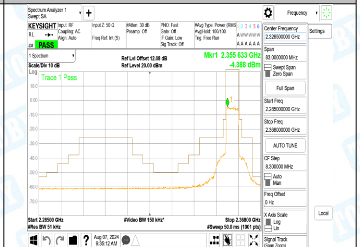
Band40_10MHz_QPSK_39200_1RB#49
