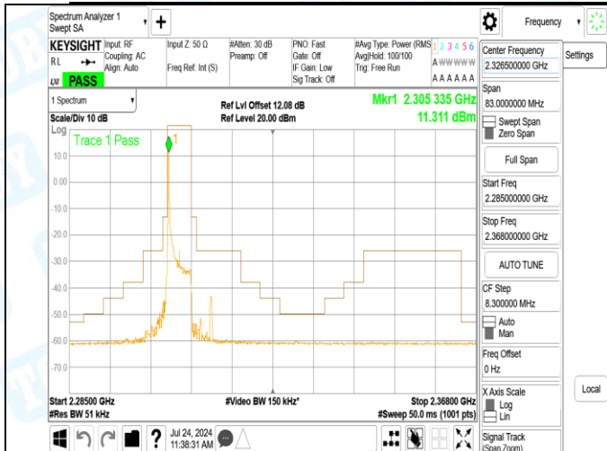
Band40_5MHz_16QAM_38725_25RB#0
