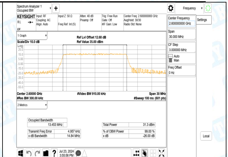
41(2555-2655)-15MHz-16QAM-40315-75RB#0-PASS
