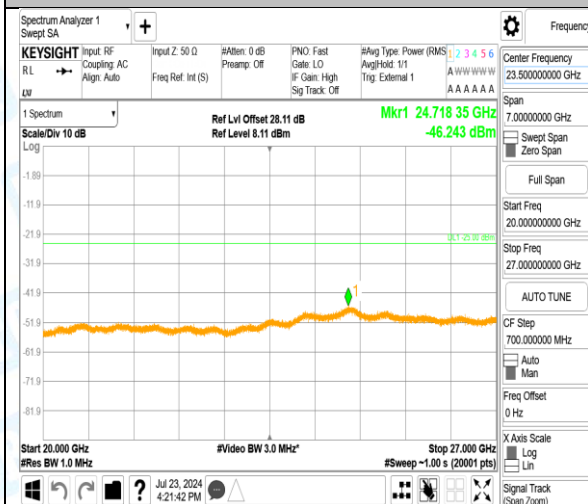
Band41_20MHz_QPSK_40690_1RB#0_0.15~30_0.15~30
