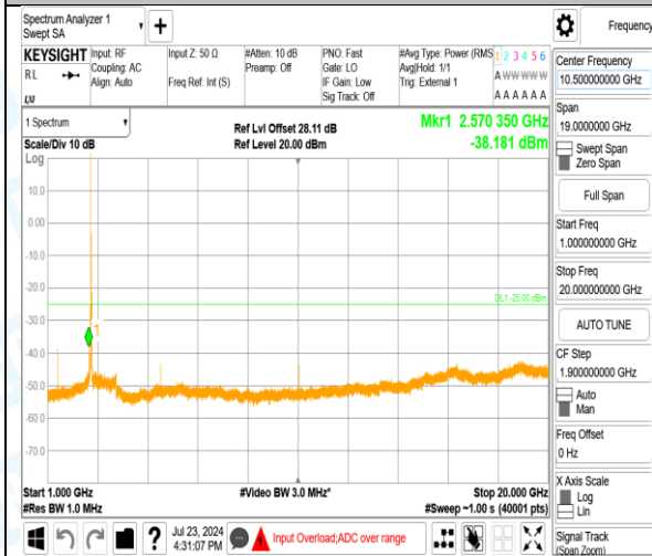
Band41_20MHz_16QAM_41140_1RB#0_1000~20000_1000~20000
