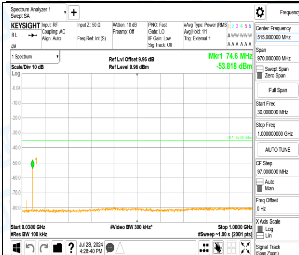
Band41_20MHz_QPSK_41140_1RB#0_20000~27000_20000~27000
