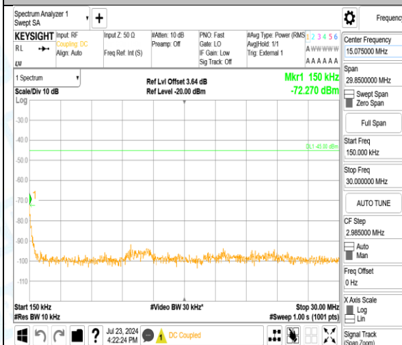
Band41_20MHz_16QAM_40340_1RB#0_1000~20000_1000~20000
