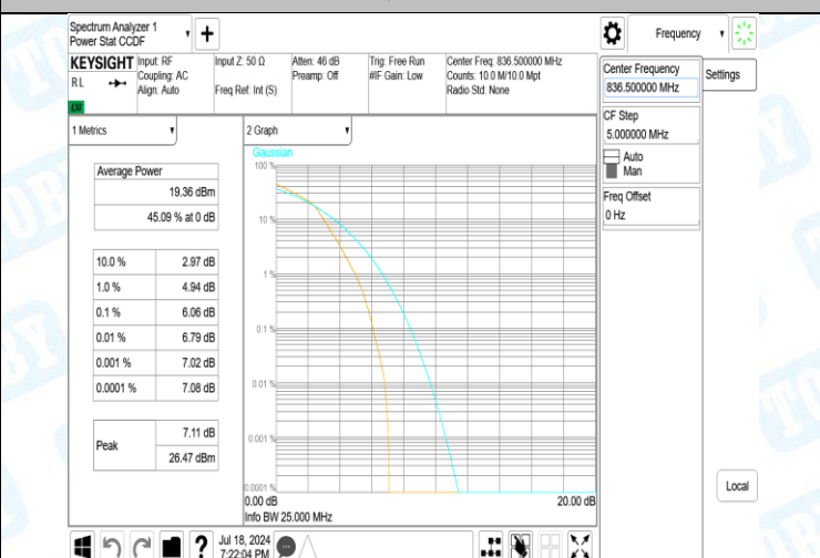
Band5-1.4MHz-16QAM-20643-6RB#0-PASS
