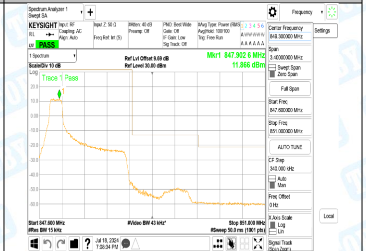
Band5_1.4MHz_16QAM_20643_6RB#0
