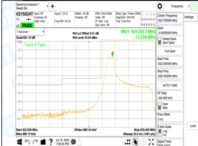
Band5_1.4MHz_16QAM_20407_6RB#0
