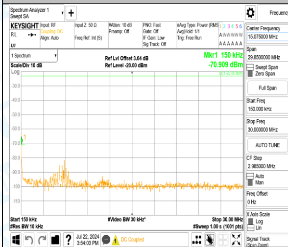
Band5_3MHz_16QAM_20635_1RB#0_1000~3000_1000~3000
