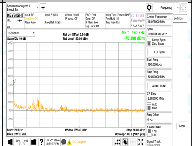
Band5_3MHz_QPSK_20635_1RB#0_1000~3000_1000~3000
