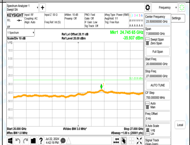
Band7_5MHz_QPSK_21425_1RB#0_0.15~30_0.15~30
