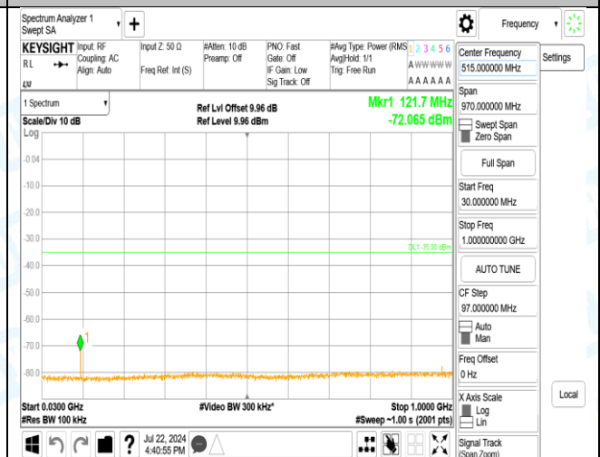
Band7_5MHz_16QAM_20775_1RB#0_20000~27000_20000~27000
