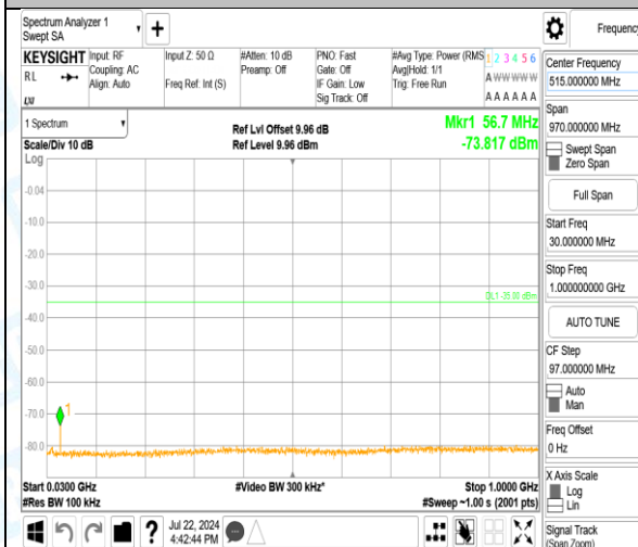
Band7_5MHz_16QAM_21100_1RB#0_20000~27000_20000~27000
