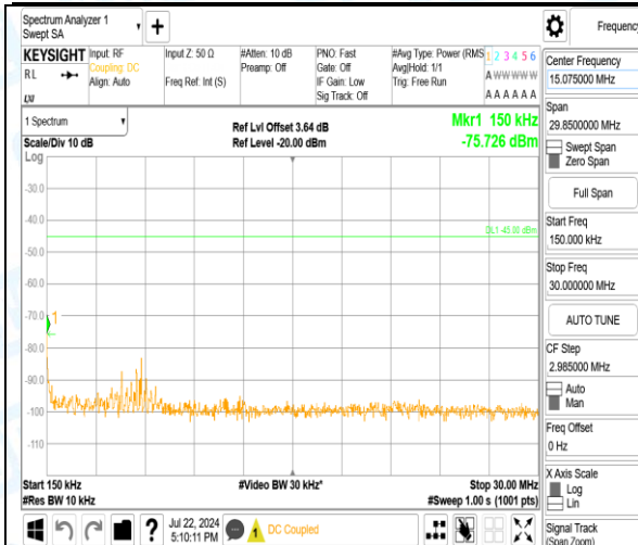
Band7_15MHz_QPSK_21100_1RB#0_1000~20000_1000~20000
