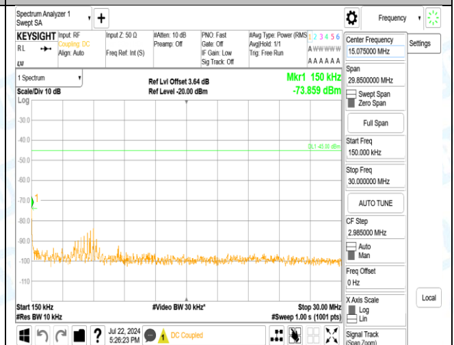
Band7_20MHz_QPSK_21350_1RB#0_1000~20000_1000~20000
