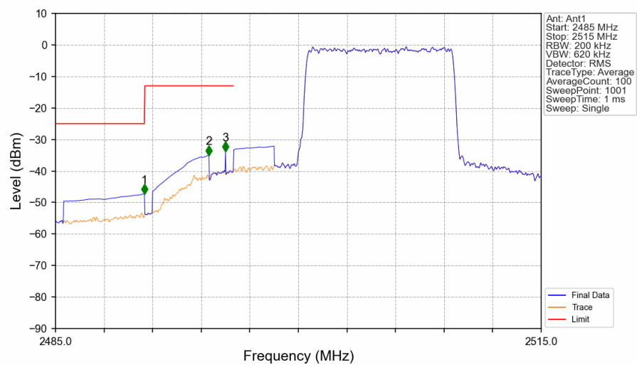
Band7_10MHz_16QAM_LCH_2505MHz_RB_50_0_NTNV
