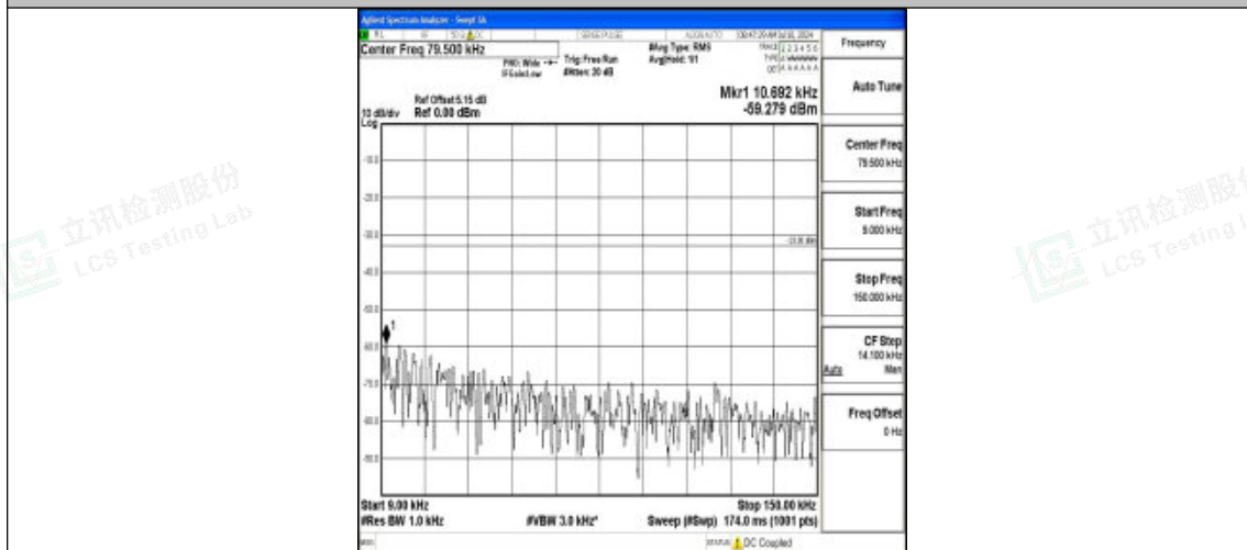
Band5_10MHz_QPSK_20525_1RB#0_0.009~0.15_0.009~0.15
