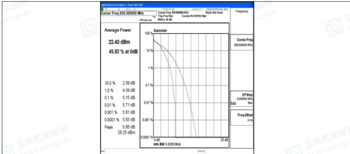
Band5-5MHz-QPSK-20525-1RB#0-PASS
