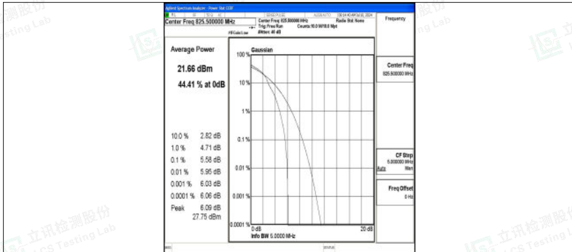
Band5-3MHz-16QAM-20415-1RB#0-PASS
