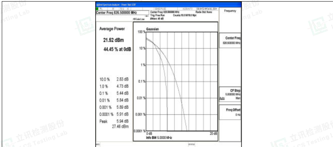
Band5-5MHz-16QAM-20425-1RB#0-PASS
