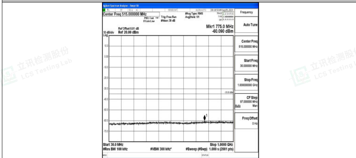
Band7-20MHz-QPSK-21350-1RB#0-30~1000-PASS
