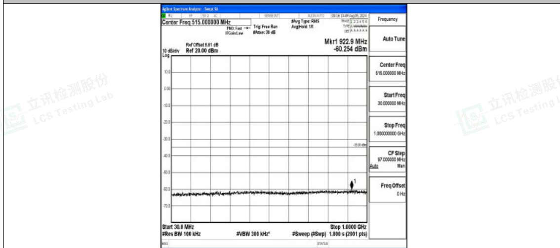
Band7-20MHz-QPSK-21100-1RB#0-30~1000-PASS
