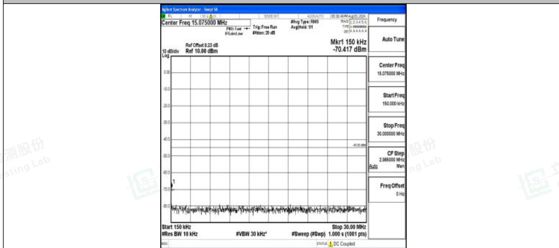
Band7-10MHz-QPSK-21100-1RB#0-0.15~30-PASS
