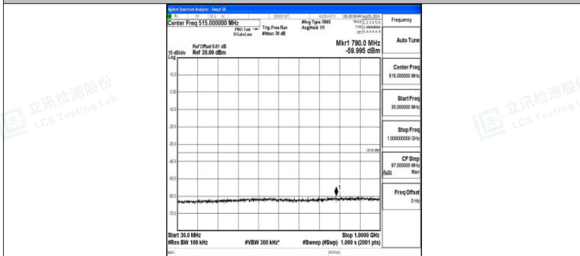
Band7-20MHz-16QAM-21350-1RB#0-30~1000-PASS
