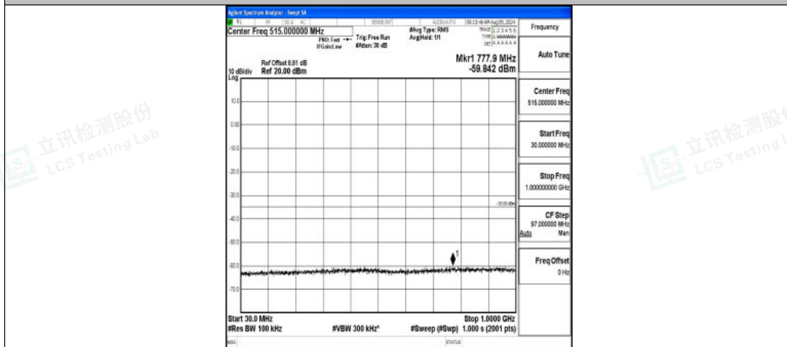
Band7-20MHz-QPSK-20850-1RB#0-30~1000-PASS
