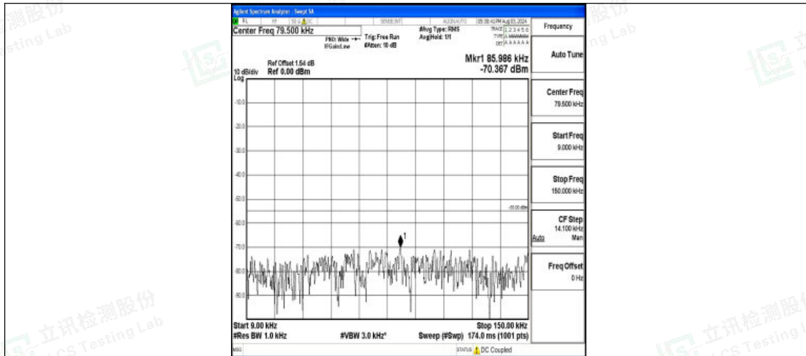
Band7-10MHz-QPSK-21100-1RB#0-0.009~0.15-PASS
