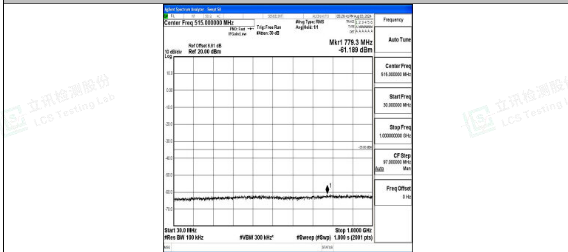
Band7-10MHz-16QAM-20800-1RB#0-30~1000-PASS
