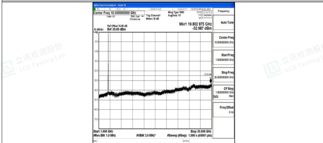
Band41_15MHz_QPSK_40620_1RB#0_1000~20000_1000~20000
