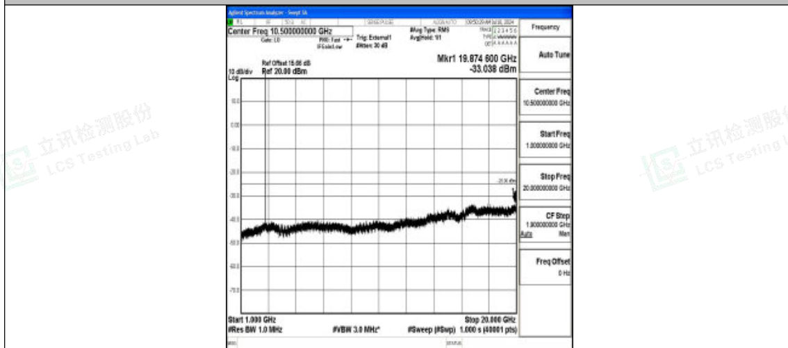
Band41_10MHz_16QAM_41540_1RB#0_1000~20000_1000~20000
