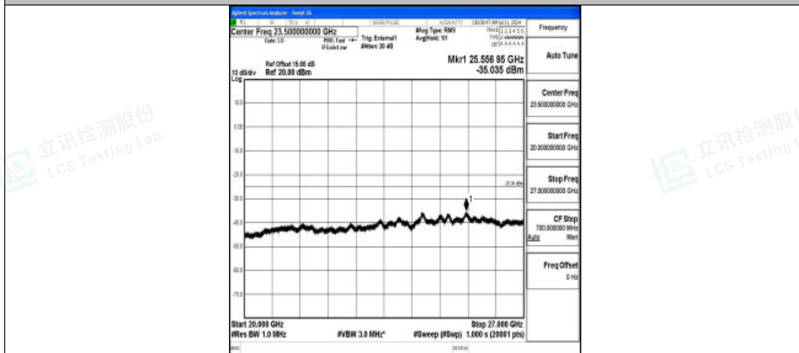
Band41_20MHz_16QAM_40620_1RB#0_20000~27000_20000~27000
