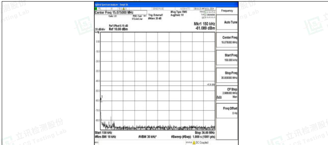
Band41_20MHz_16QAM_41490_1RB#0_0.15~30_0.15~30
