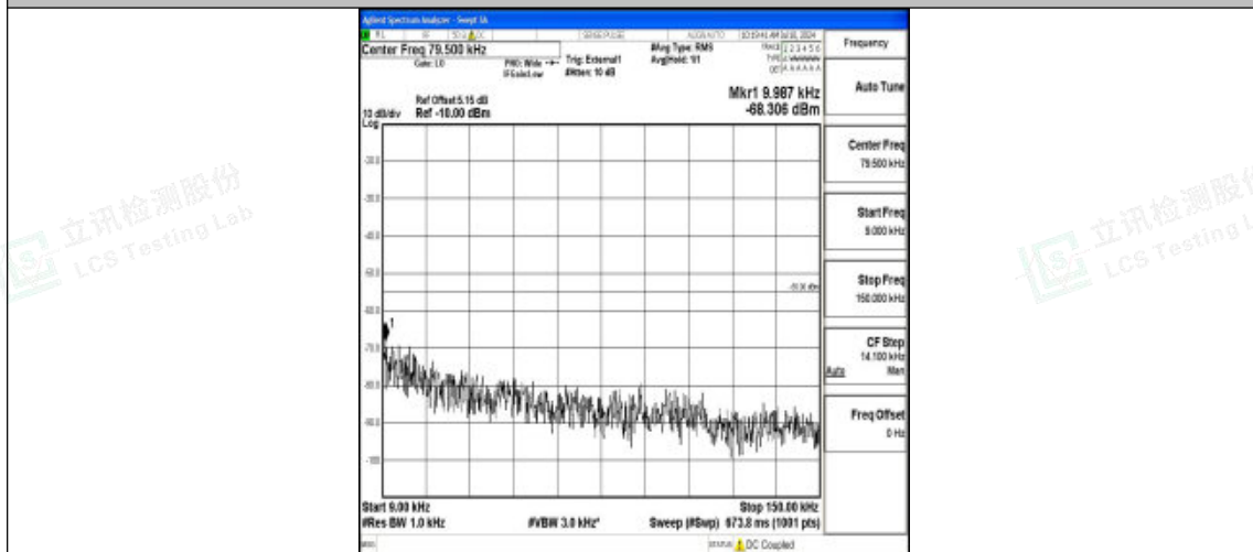
Band41_15MHz_16QAM_41515_1RB#0_0.009~0.15_0.009~0.15
