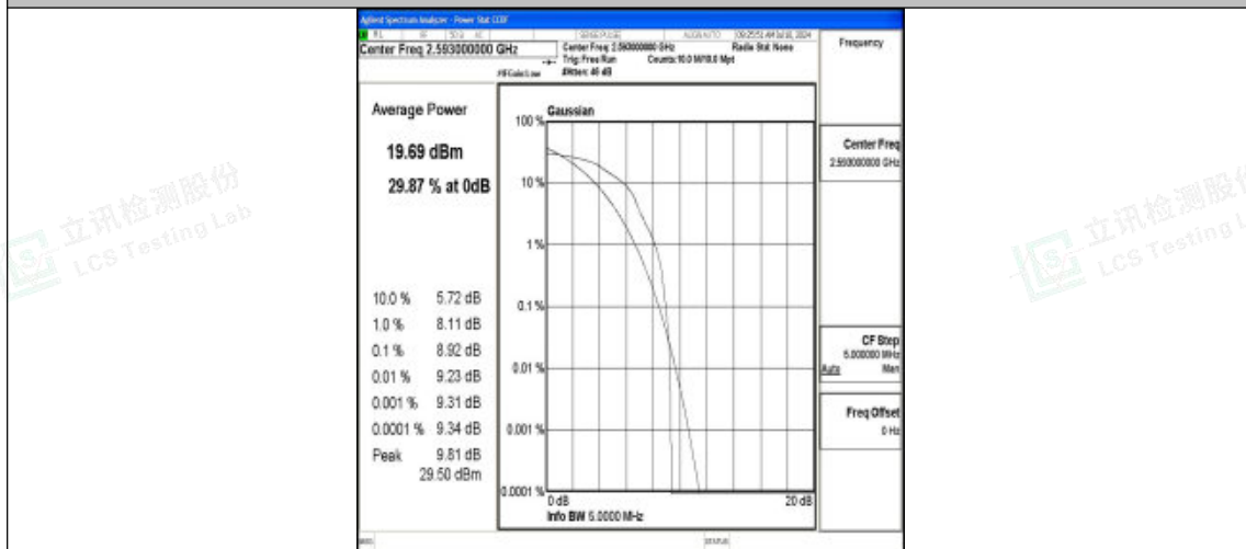
Band41-5MHz-16QAM-40620-1RB#0-PASS
