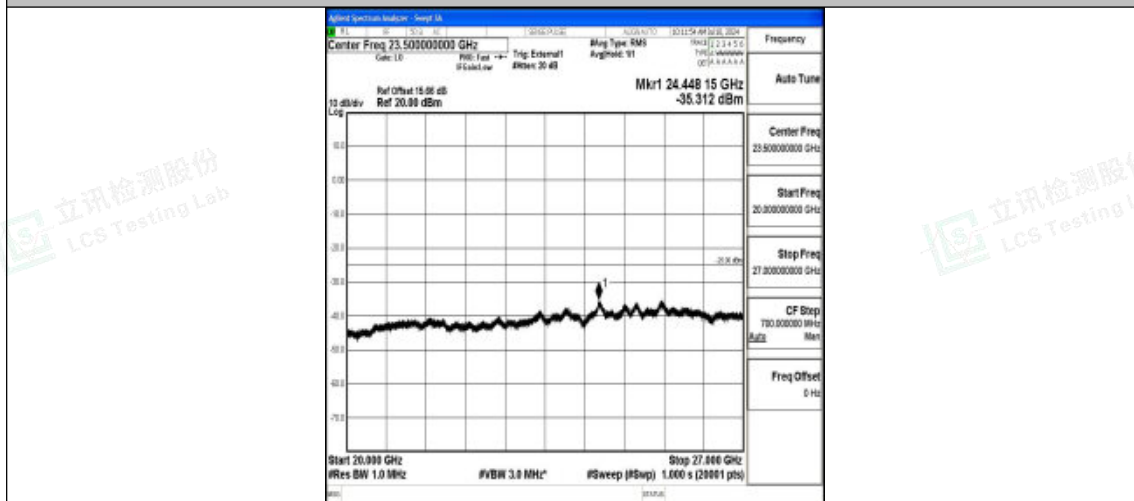
Band41_15MHz_QPSK_39725_1RB#0_20000~27000_20000~27000
