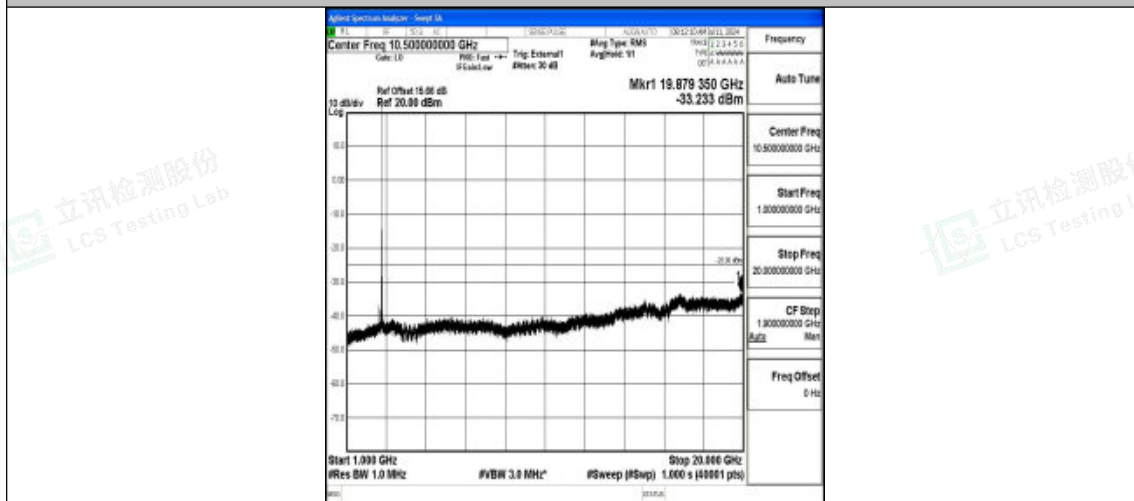
Band41_20MHz_16QAM_41490_1RB#0_1000~20000_1000~20000
