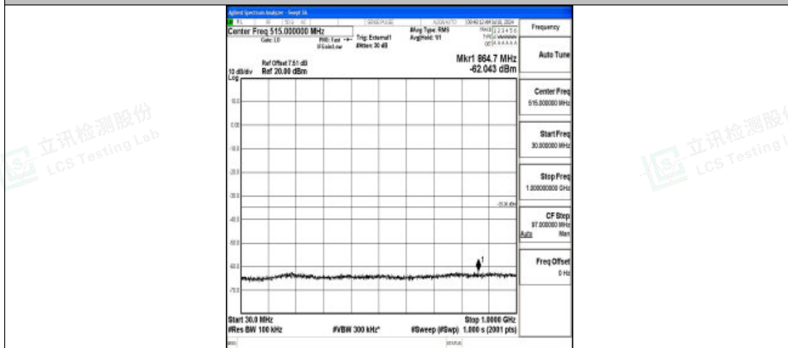
Band41_10MHz_QPSK_41540_1RB#0_30~1000_30~1000
