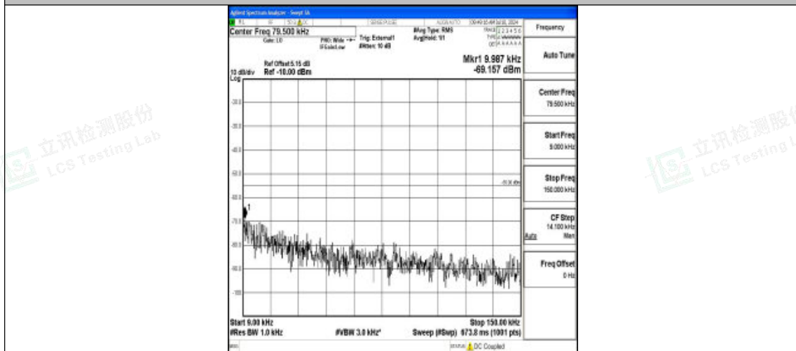
Band41_10MHz_16QAM_41540_1RB#0_0.009~0.15_0.009~0.15
