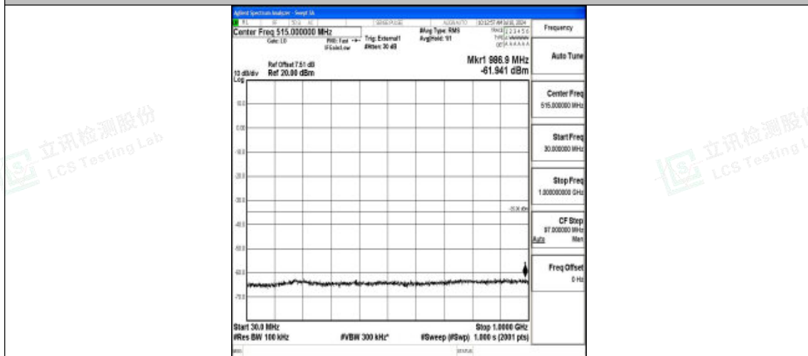
Band41_15MHz_16QAM_39725_1RB#0_30~1000_30~1000
