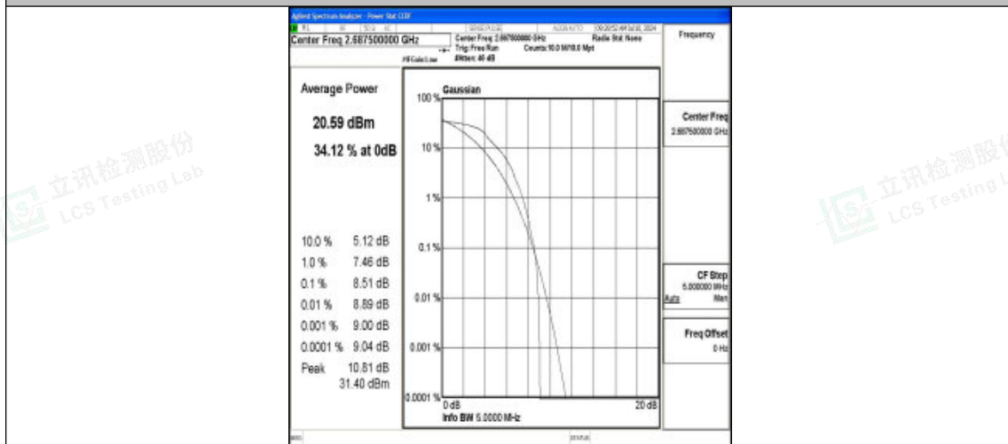
Band41-5MHz-QPSK-41565-1RB#0-PASS
