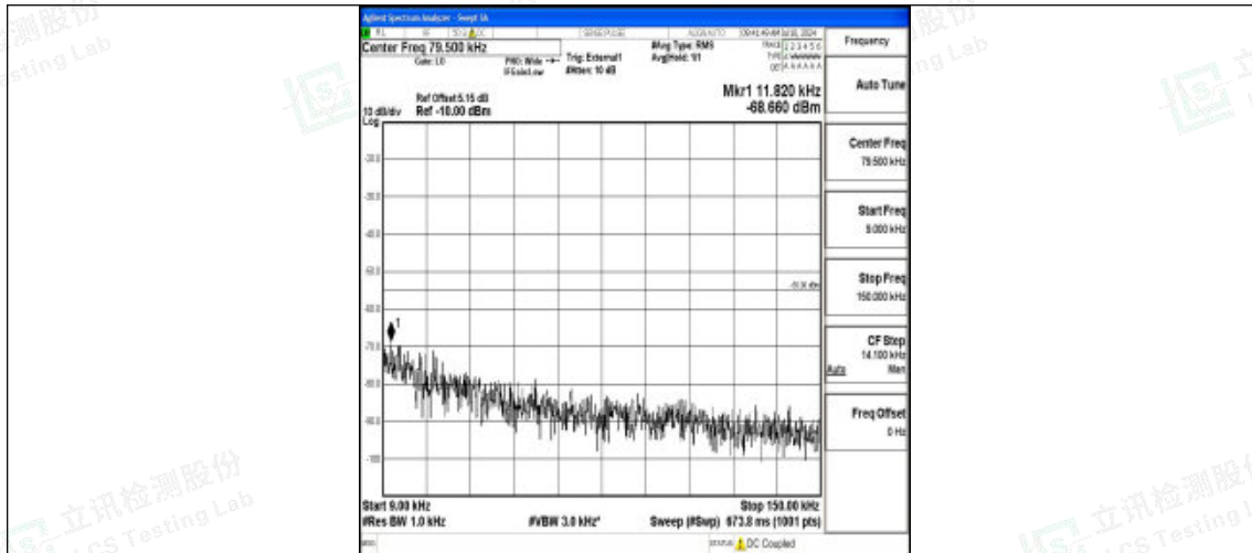
Band41_10MHz_16QAM_39700_1RB#0_0.009~0.15_0.009~0.15
