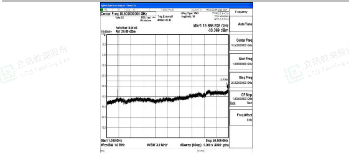
Band41_5MHz_16QAM_41565_1RB#0_1000~20000_1000~20000
