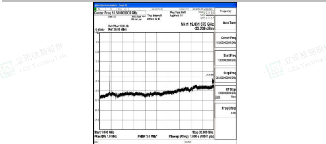
Band41_15MHz_16QAM_41515_1RB#0_1000~20000_1000~20000
