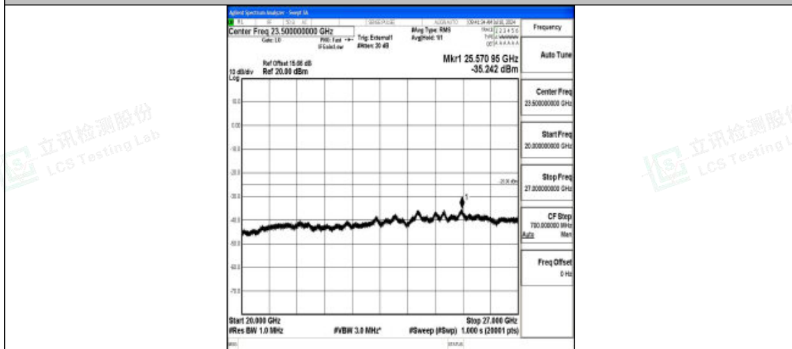
Band41_10MHz_QPSK_39700_1RB#0_20000~27000_20000~27000
