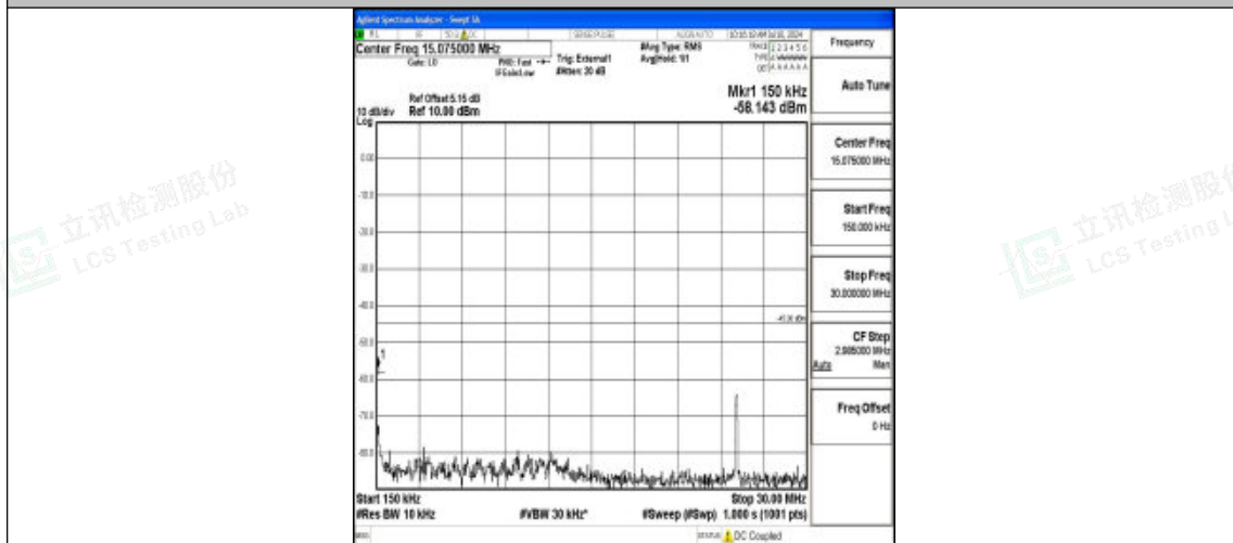
Band41_15MHz_16QAM_40620_1RB#0_0.15~30_0.15~30
