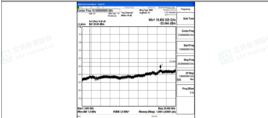
Band41_10MHz_QPSK_40620_1RB#0_1000~20000_1000~20000
