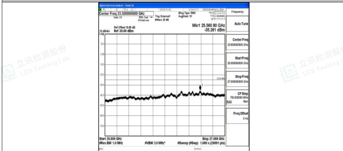
Band41_20MHz_QPSK_39750_1RB#0_20000~27000_20000~27000
