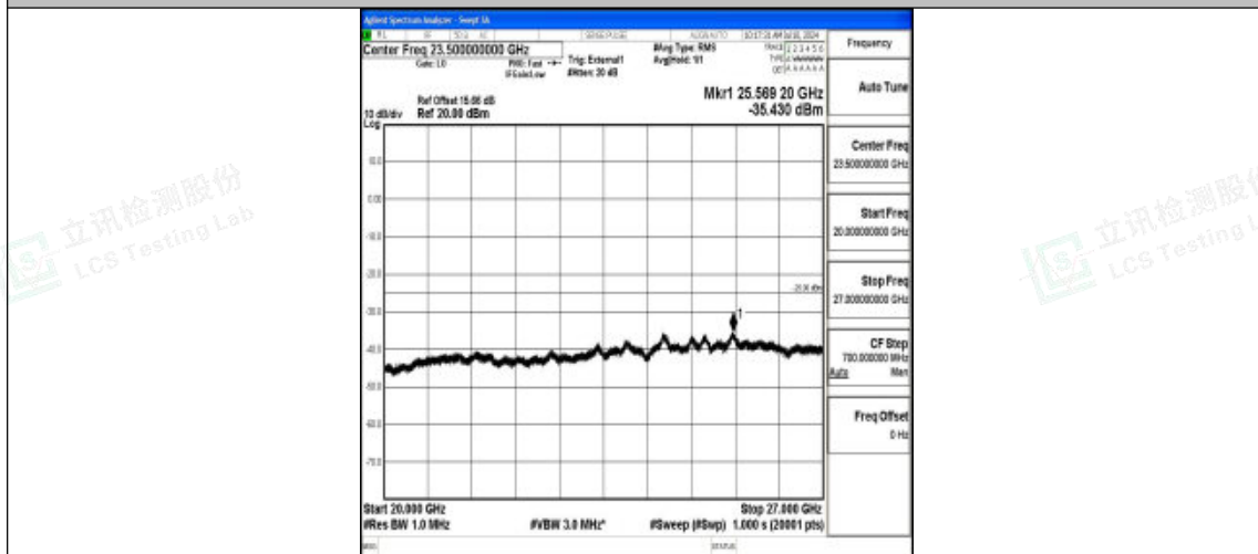
Band41_15MHz_16QAM_40620_1RB#0_20000~27000_20000~27000
