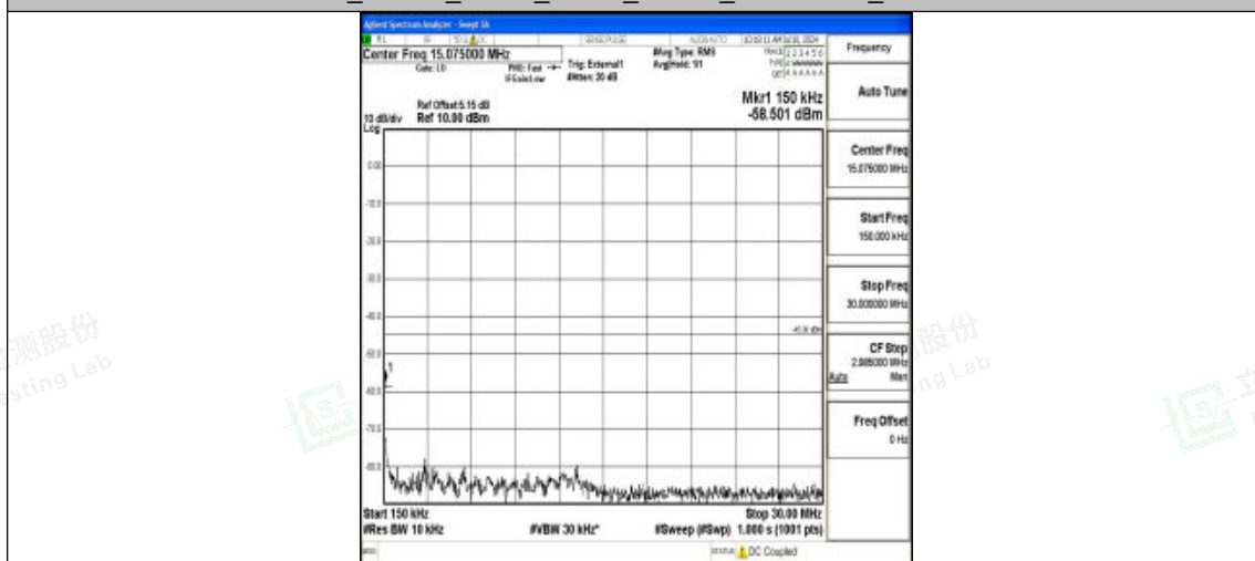
Band41_15MHz_QPSK_41515_1RB#0_0.15~30_0.15~30
