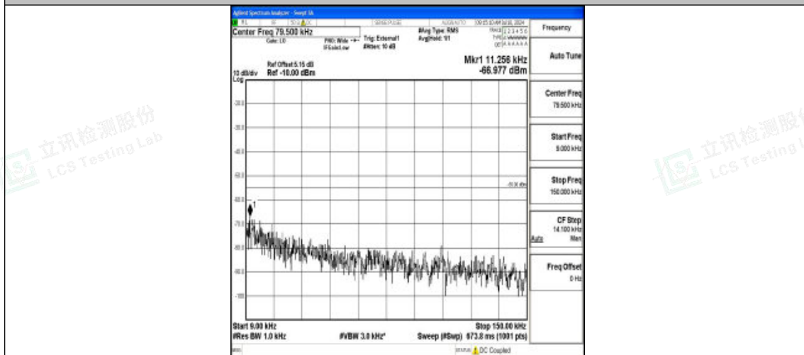
Band41_5MHz_16QAM_41565_1RB#0_0.009~0.15_0.009~0.15
