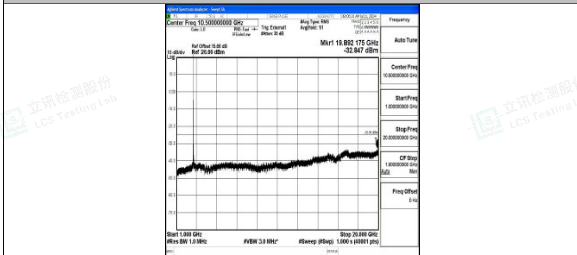
Band41_20MHz_QPSK_40620_1RB#0_1000~20000_1000~20000
