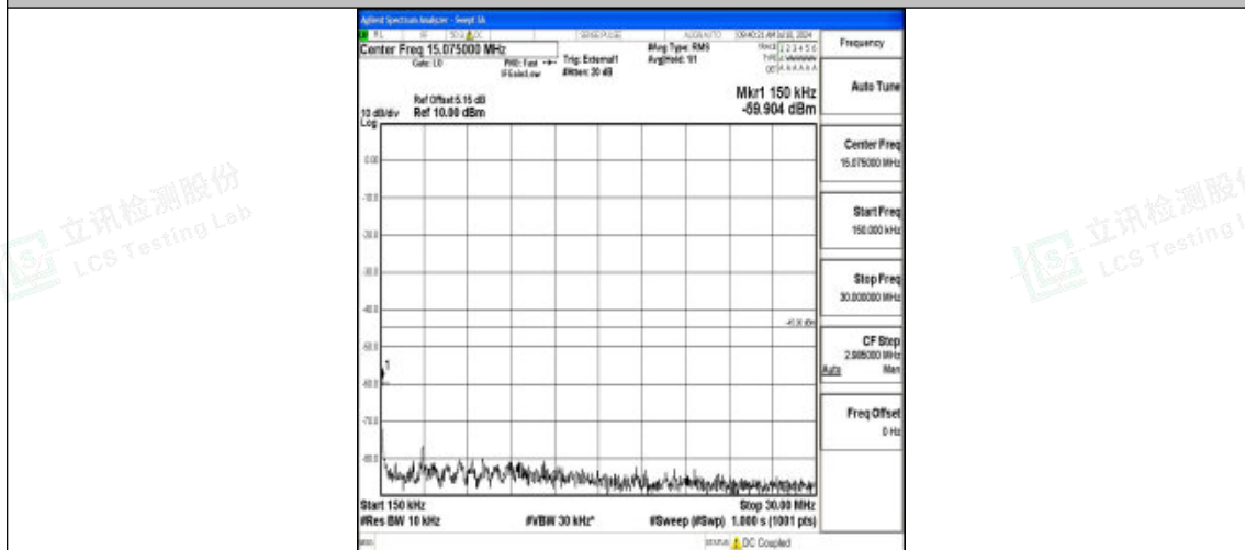
Band41_10MHz_QPSK_39700_1RB#0_0.15~30_0.15~30
