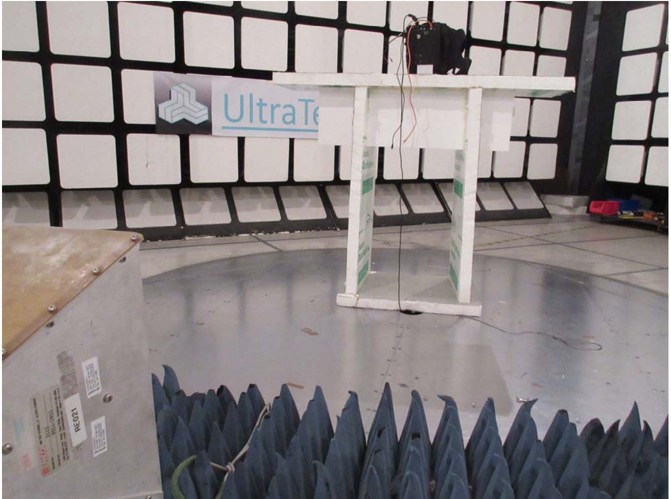
Radiated Emissions at 3 m
