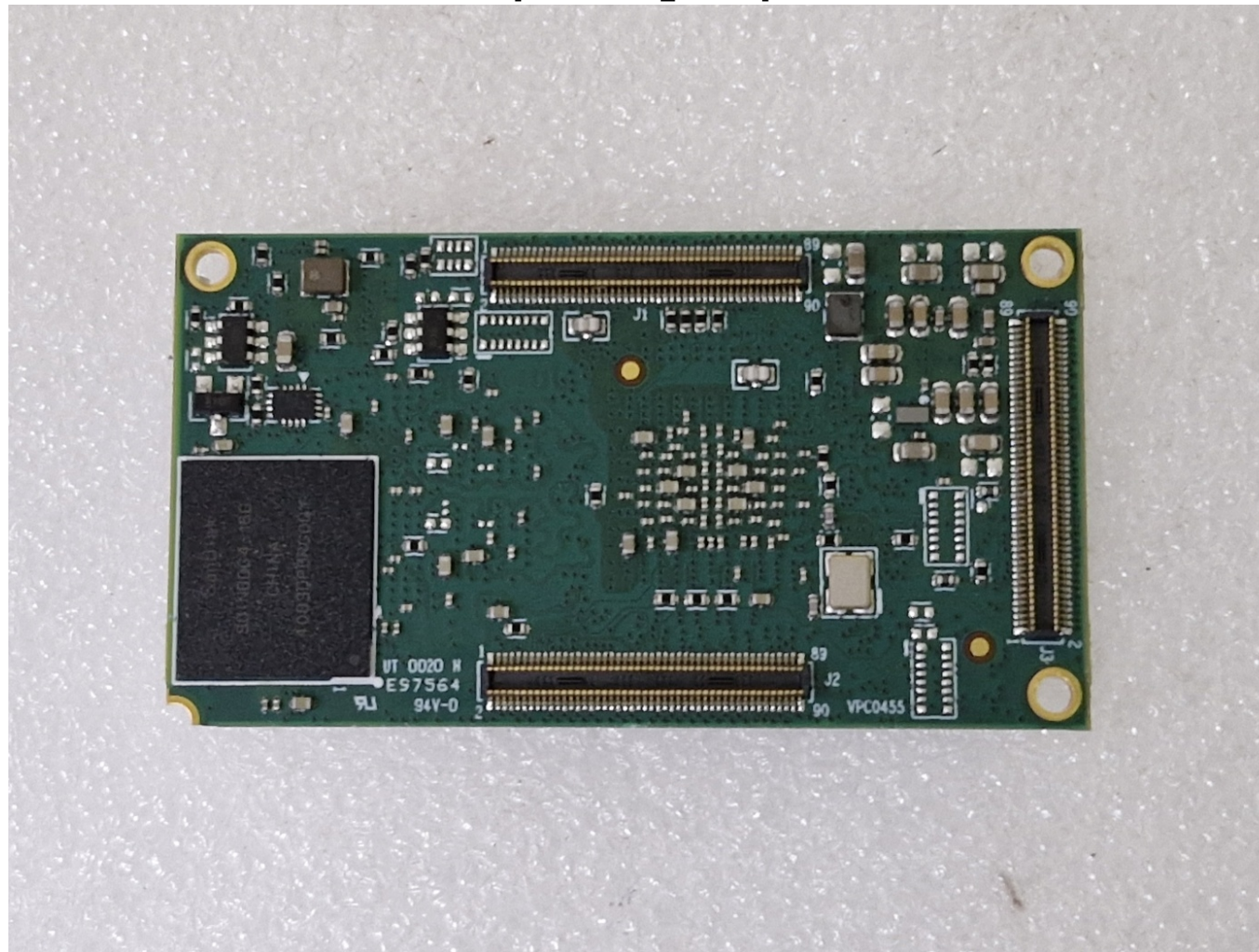
[Sub Board1_Bottom]
