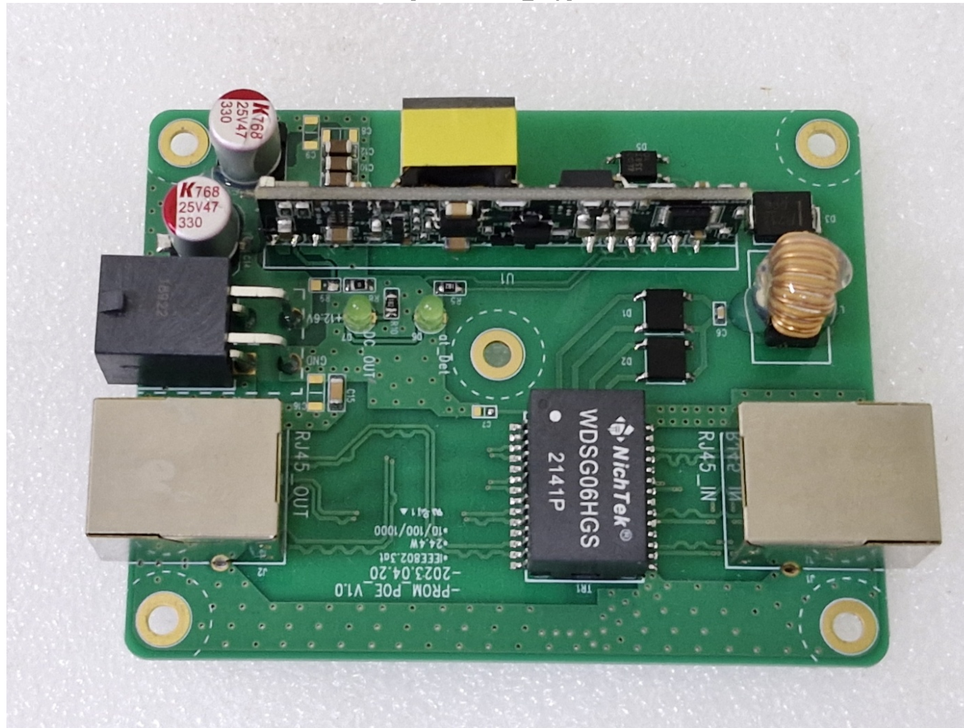
[Sub Board2_Top]
