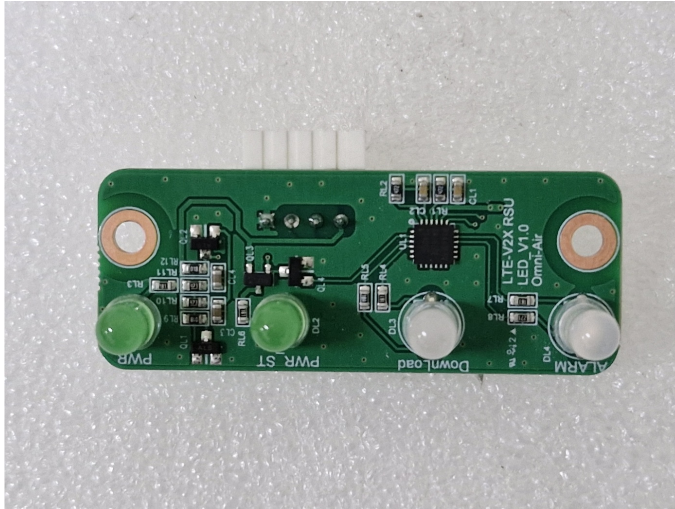
[LED Board_Top]
