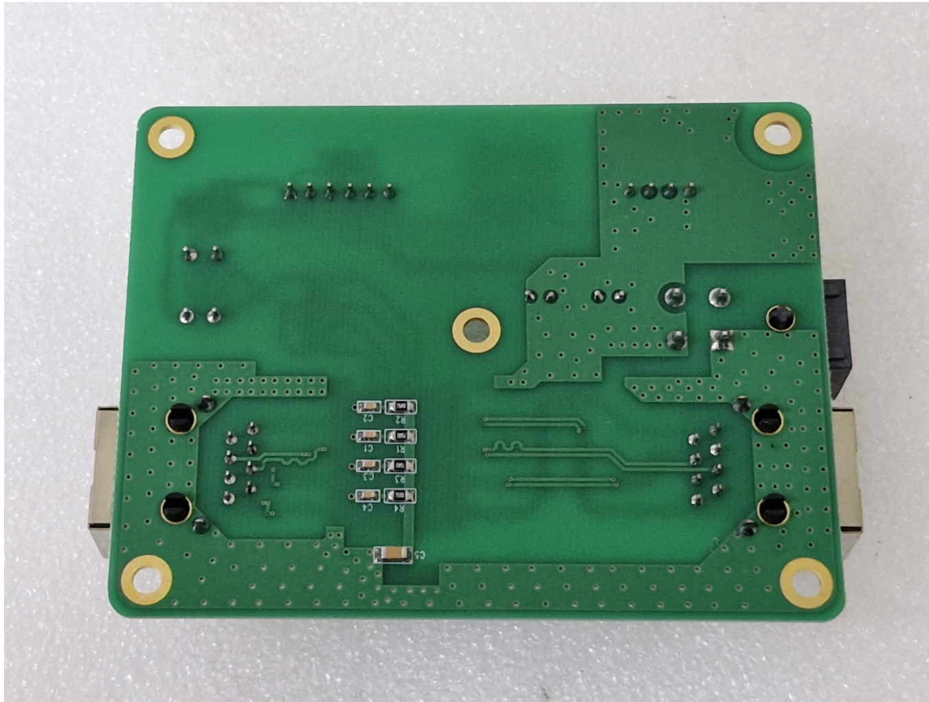
[Sub Board2_Bottom]
