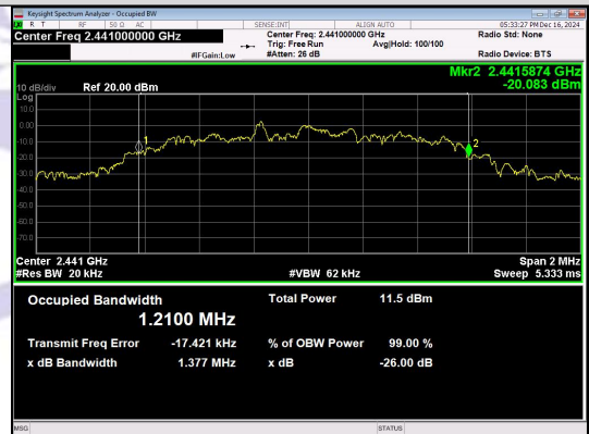
n/4DQPSK_2-DH1_Channel 39
