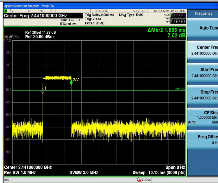
3DH3-Ant1-Hop-PASS
