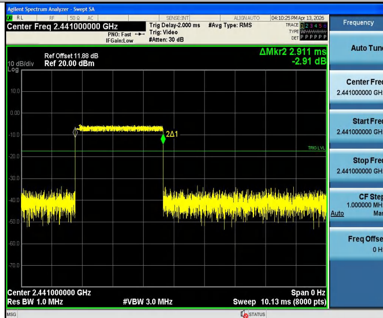
3DH5-Ant1-Hop-PASS
