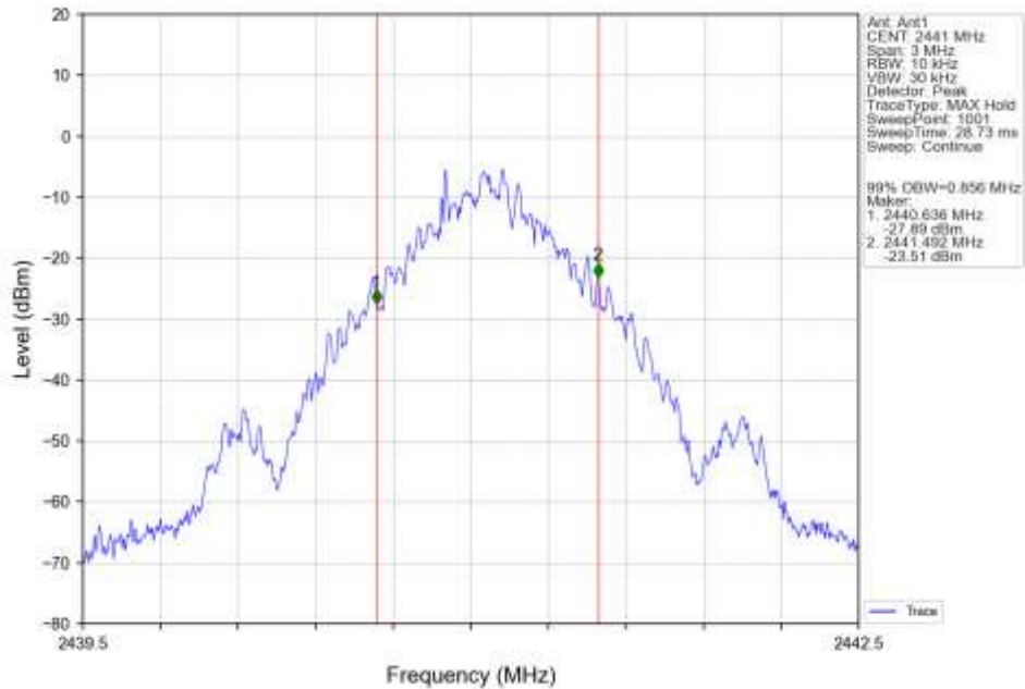
GFSK_DH5_MCH_2441MHz_Ant1_NTNV
