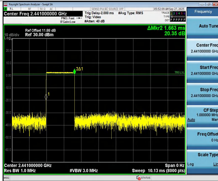
2DH3-Ant1-Hop-PASS
