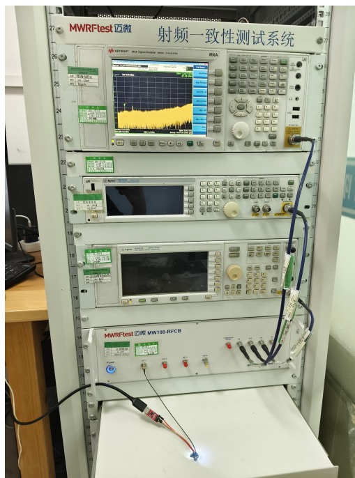
RF Conduction
