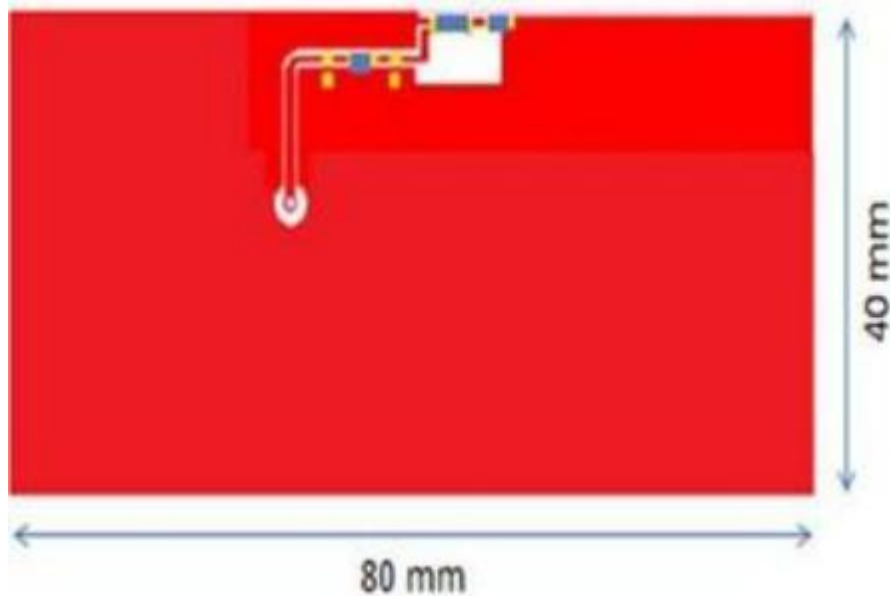
Evaluation Board and Matching Circuits
