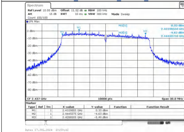
IEEE 802.11g Channel 6_20MHz_Antenna 1
