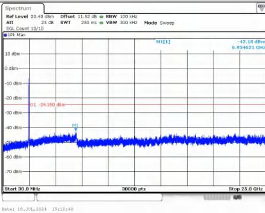
30.0 MHz - 25000.0 MHz IEEE 802.11ax_Channel 6_40MHz_Antenna 1_RU&Index SU
