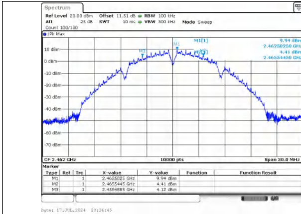
IEEE 802.11b Channel 11_20MHz_Antenna 1
