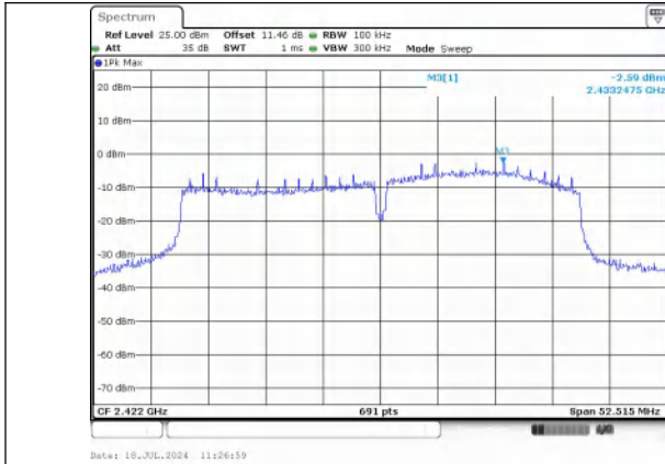
In-Band Reference Level IEEE 802.11n_Channel 3_40MHz_Antenna 1
