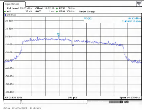
In-Band Reference Level IEEE 802.11n Channel 6_20MHz_Antenna 1
