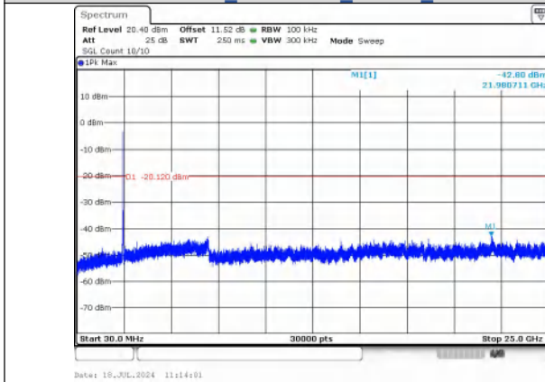
30.0 MHz - 25000.0 MHz IEEE 802.11n Channel 6_20MHz_Antenna 1
