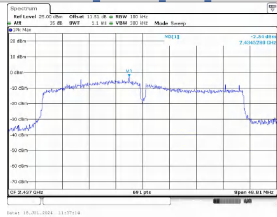
In-Band Reference Level IEEE 802.11n_Channel 6_40MHz_Antenna 1
