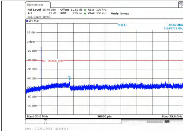
30.0 MHz - 25000.0 MHz IEEE 802.11n Channel 1_20MHz_Antenna 1
