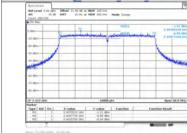
IEEE 802.11n Channel 1_20MHz_Antenna 1
