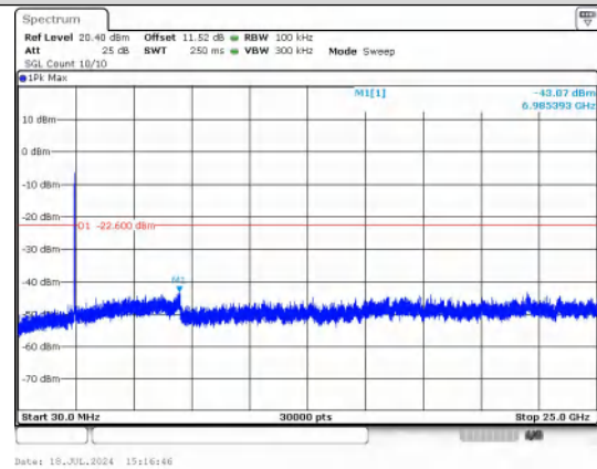
30.0 MHz - 25000.0 MHz IEEE 802.11ax_Channel 9_40MHz_Antenna 1_RU&Index SU
