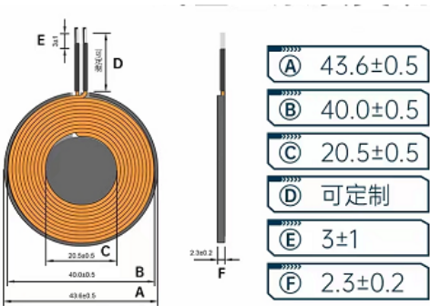
Antenna Top View [With Ruler]
