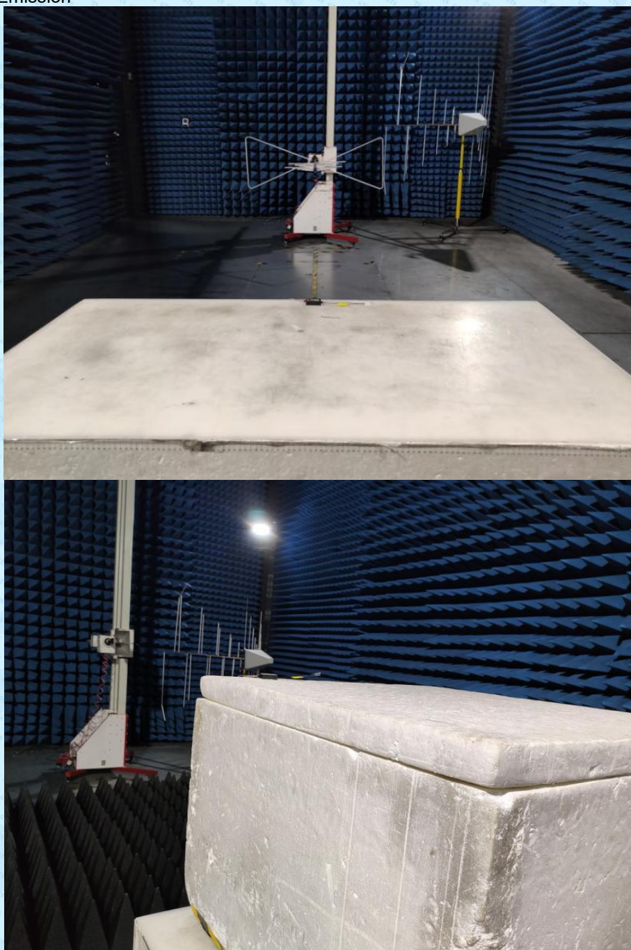
Radiated Emission
