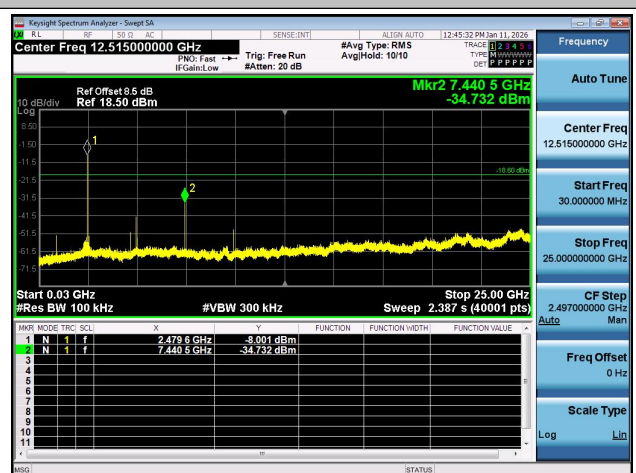
2.4G SRD-Ant1-2479-30~25000-PASS
