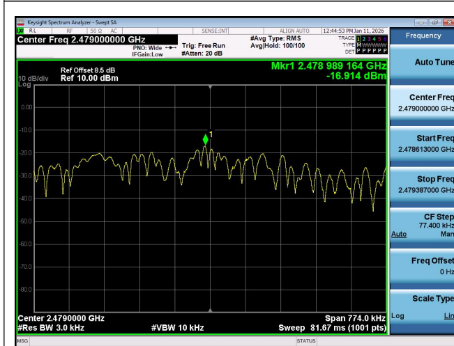
2.4G SRD-Ant1-2479-PASS
