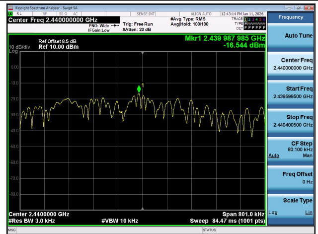
2.4G SRD-Ant1-2440-PASS
