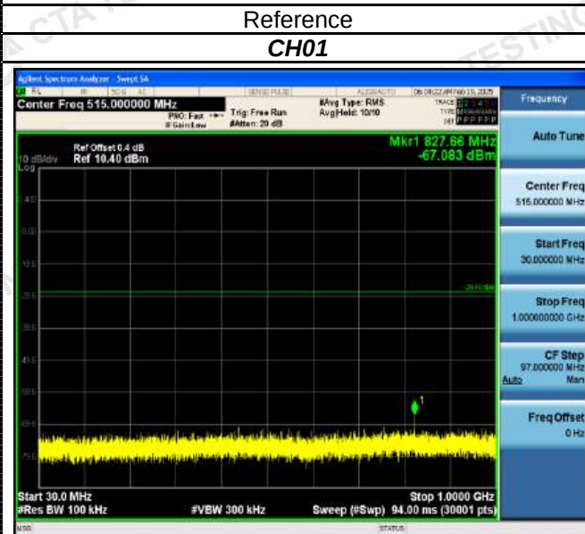
30MHz-1GHz
