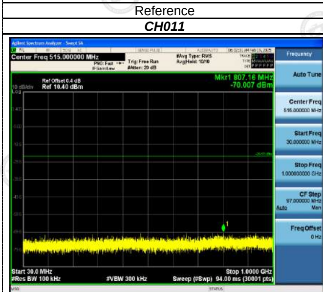
30MHz-1GHz
