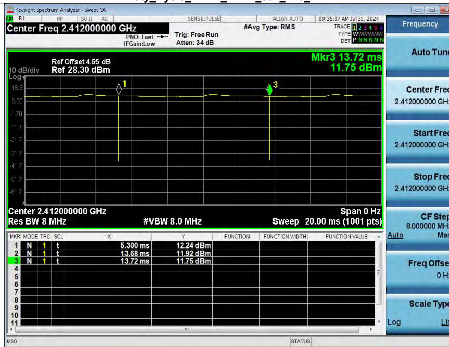
Duty_Cycle_NVNT_ANT2_802_11b_2412
