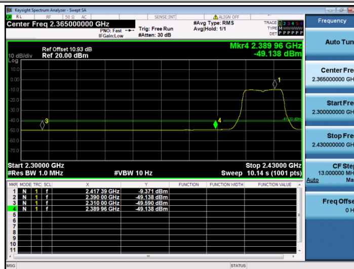
11N20SISO_Ant1_Low_2412_Peak
